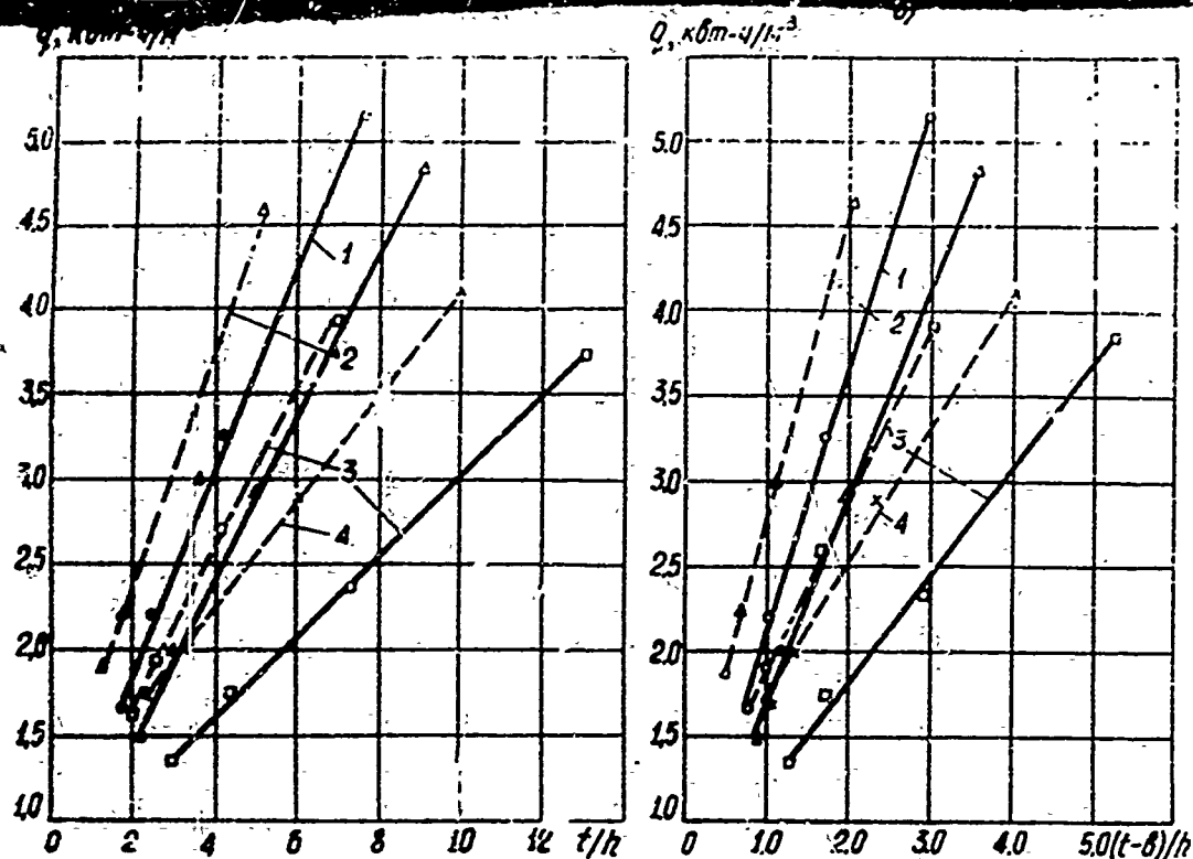
Figure 1. Relationship between specific power requirements q of bar-type cutting unit and ratios a) t/h and b) \frac{t-b}{h} when cutting frozen soil with an Ural-33 chain cutting unit with z=63 teeth (solid lines) and c=36 teeth (dashed lines) and the following cutting speeds: 1 — 1.5 m/sec; 2 — 1.8 m/sec; 3 — 2.6 m/sec; 4 — 3.5 m/sec. ZTsN cutters
