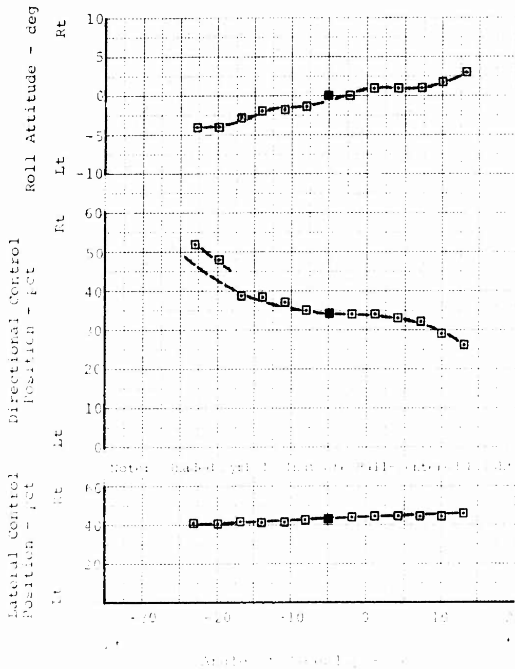
Figure D-15. Static lateral-directional stability.
