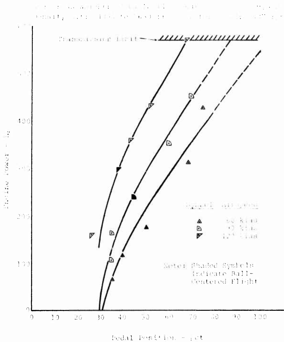
Figure D-11. Variation of pedal position with engine power.
