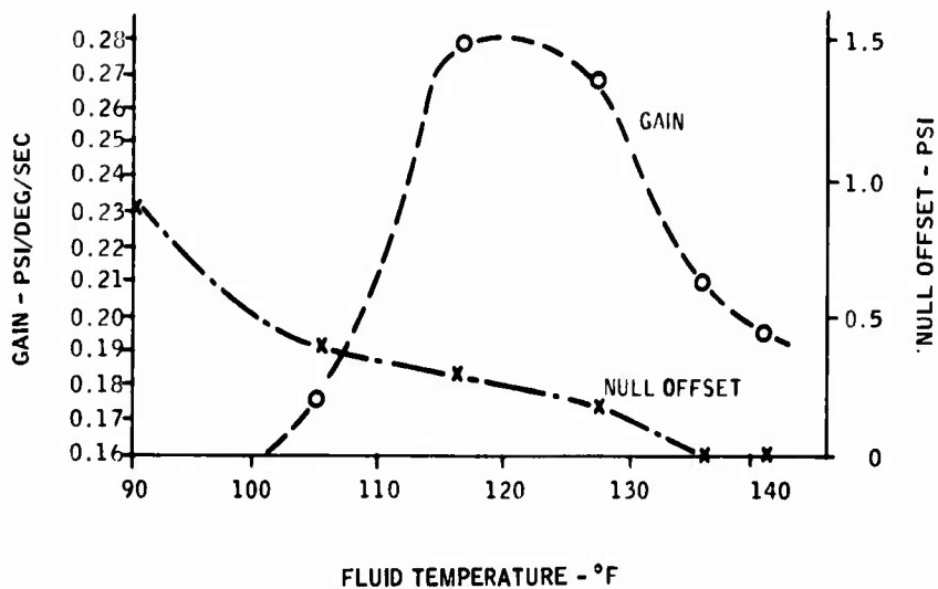
Figure 36. RAHSAS Gain Change With Oil Temperature
