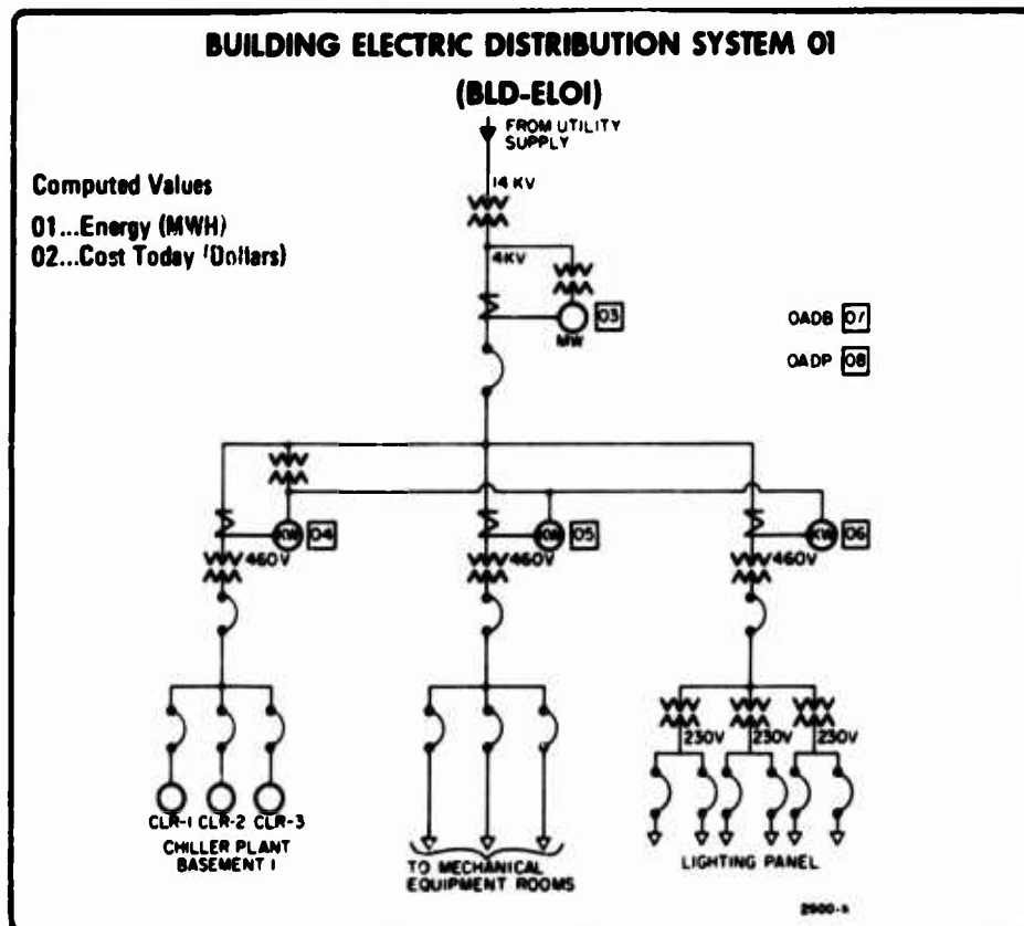
ELECTRIC DISTRIBUTION SYSTEM GRAPHIC DISPLAY
