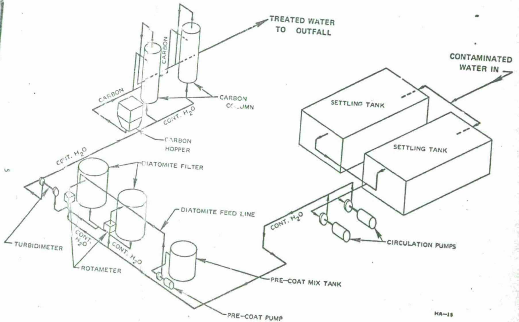
FIGURE 3 Schematic Flow Diagram - Carbon Adsorption Waste Water Treatment Plant 40 GPM Plant (IAAP)
