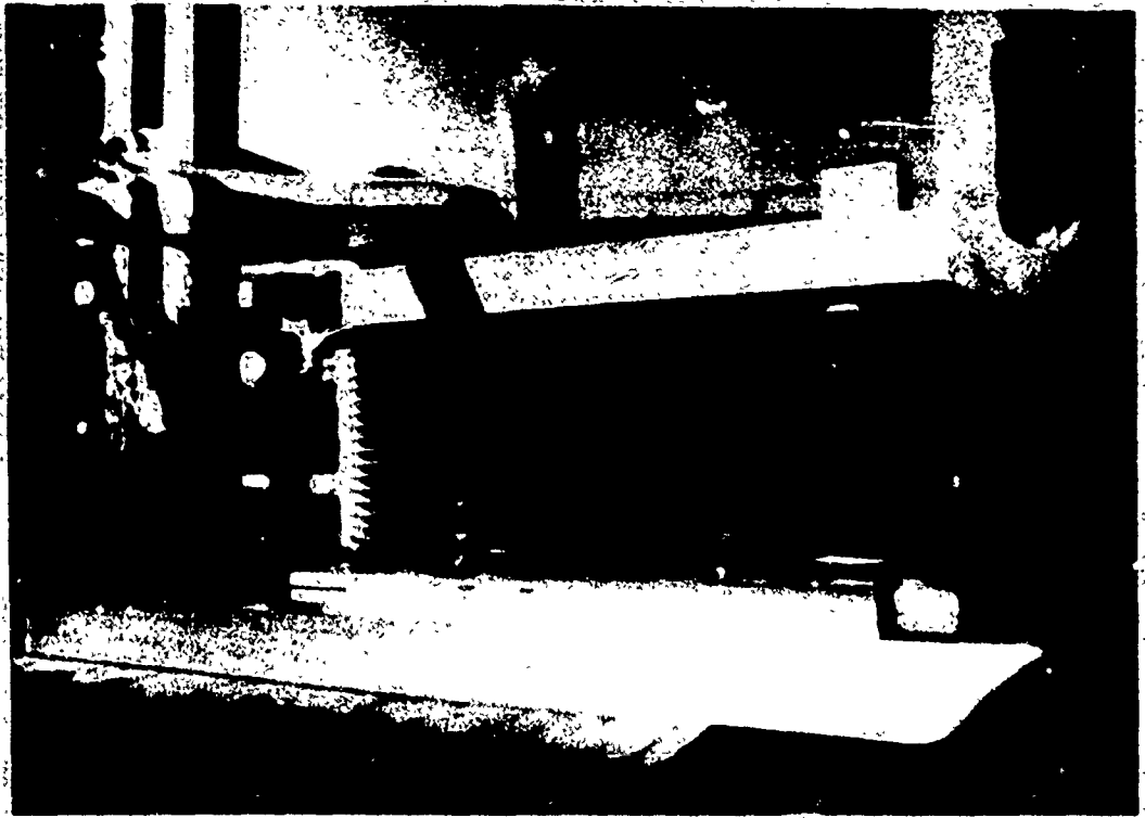
BACKREST CELL INVERTED IN TEST RIG - NOTE TANDEMLY DRIVEN BELLOWS
