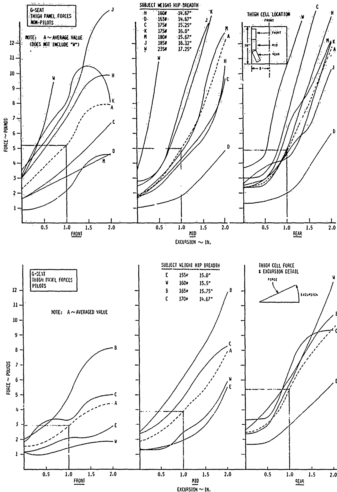
Figure 3. THIGH AREA LOADING DATA
