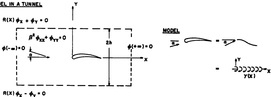
Figure 1. Boundary value problem for tunnel lift interference.
