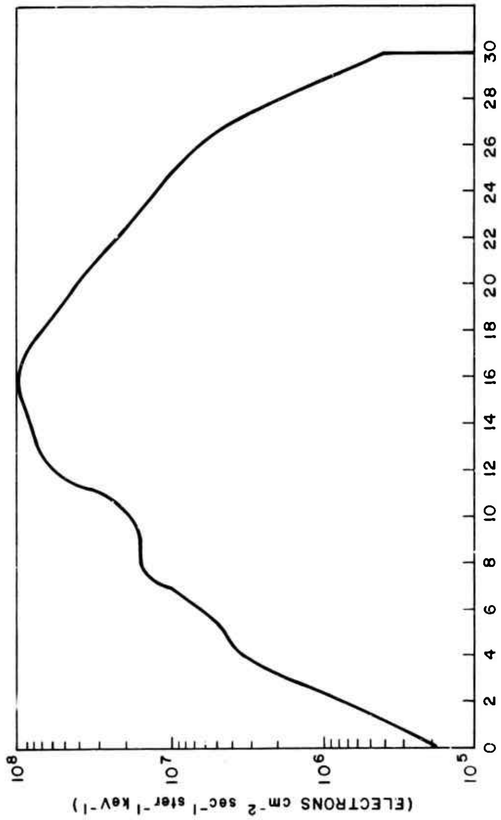
Fig. 3.1 - Assumed input electron spectrum used to exercise AURORA. This spectrum is a slightly modified ICECAP spectrum.
