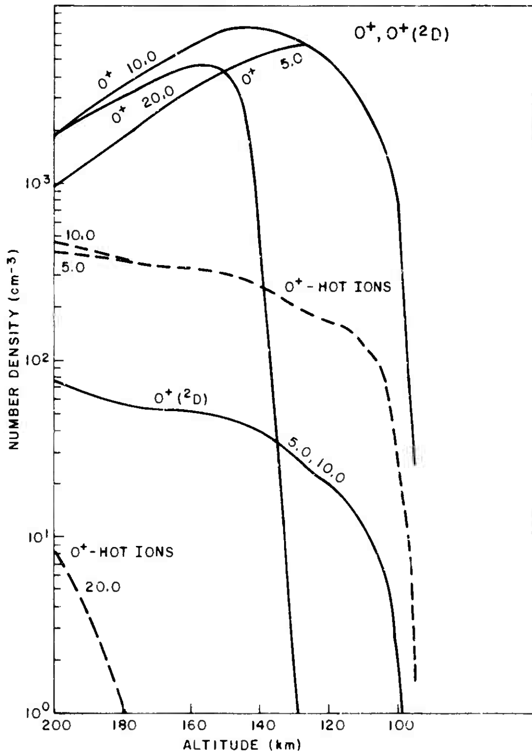
Fig. 3.2 - O^+(^1S) and O^+(^2D) profiles 5.0, 10.0 and 20.0 seconds after electron flux is turned on. Flux is turned off at 10.0 seconds.
