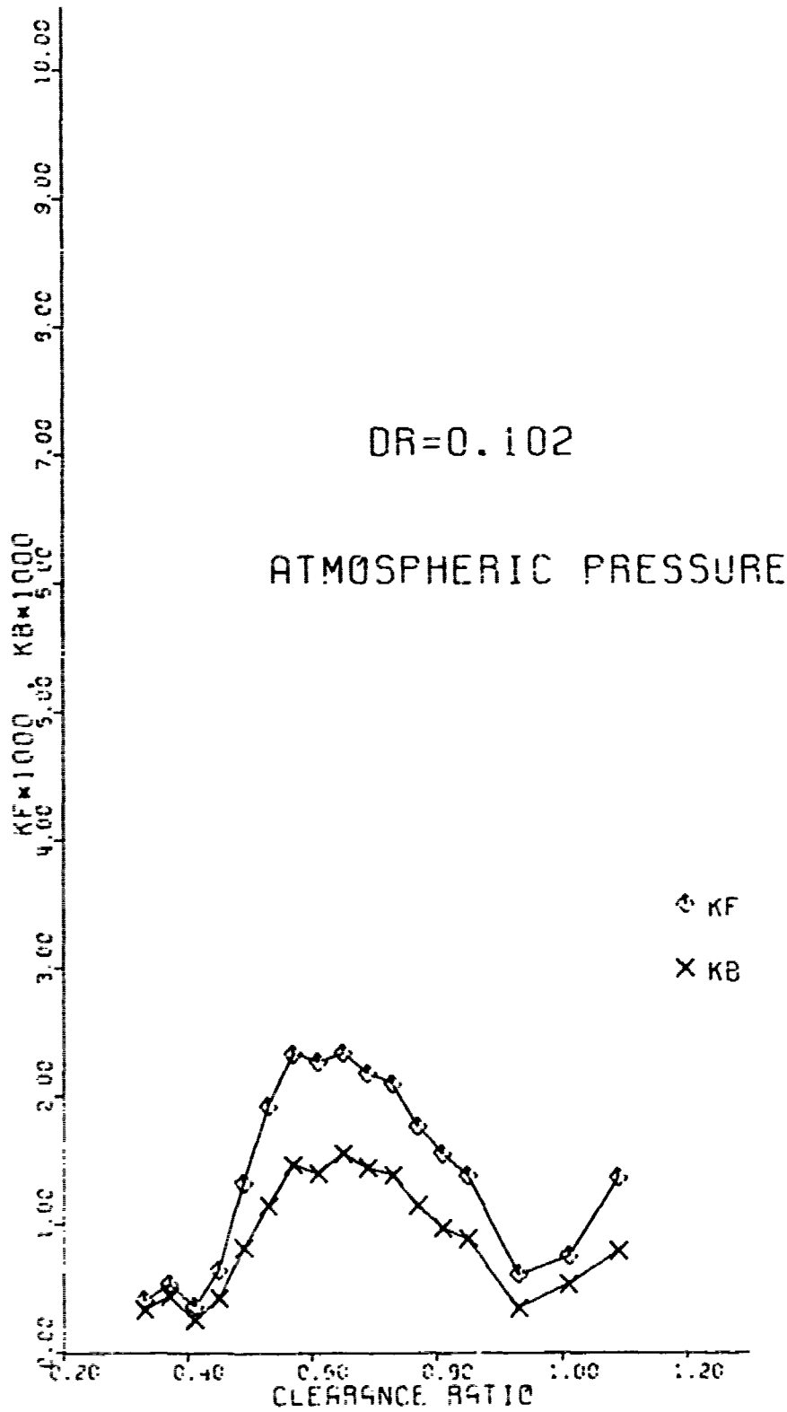
Fig. 10: Rudder vibratory loading versus clearance ratio, DR = 0.102, at atmospheric pressure.
