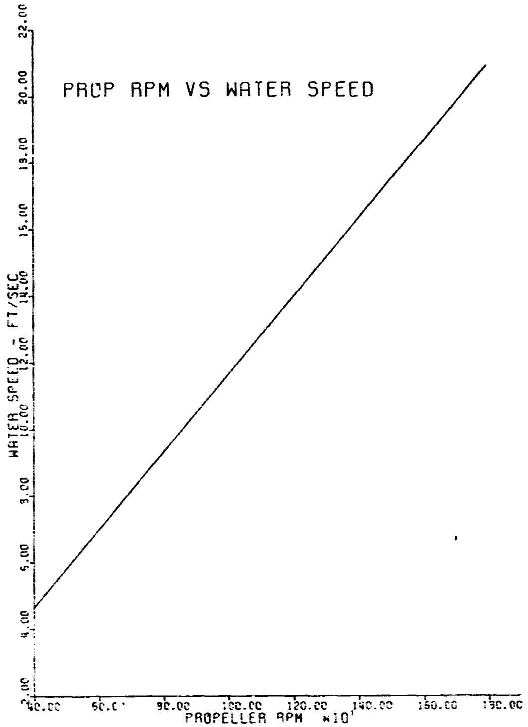
Fig.22: Propeller RPM versus tunnel water speed to simulate ship advance coefficient.
