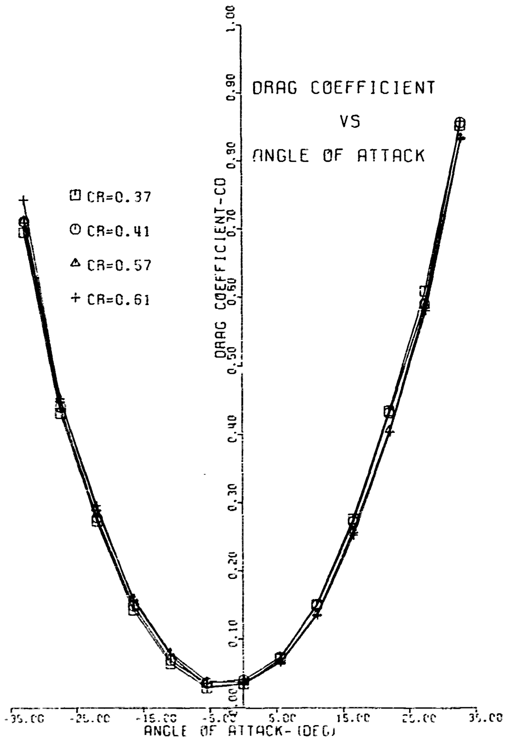
Fig. #: Rudder drag coefficient versus angle of attack for DR=.102 at four different clearance ratios. Uniform flow without cavitation, simulating J for ship.
