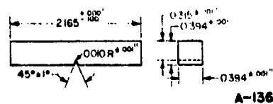
FIGURE 121. NOTCHED IMPACT SPECIMEN
