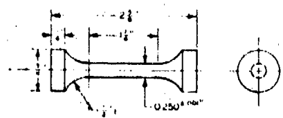
FIGURE 107. ROUND COMPRESSION SPECIMEN
