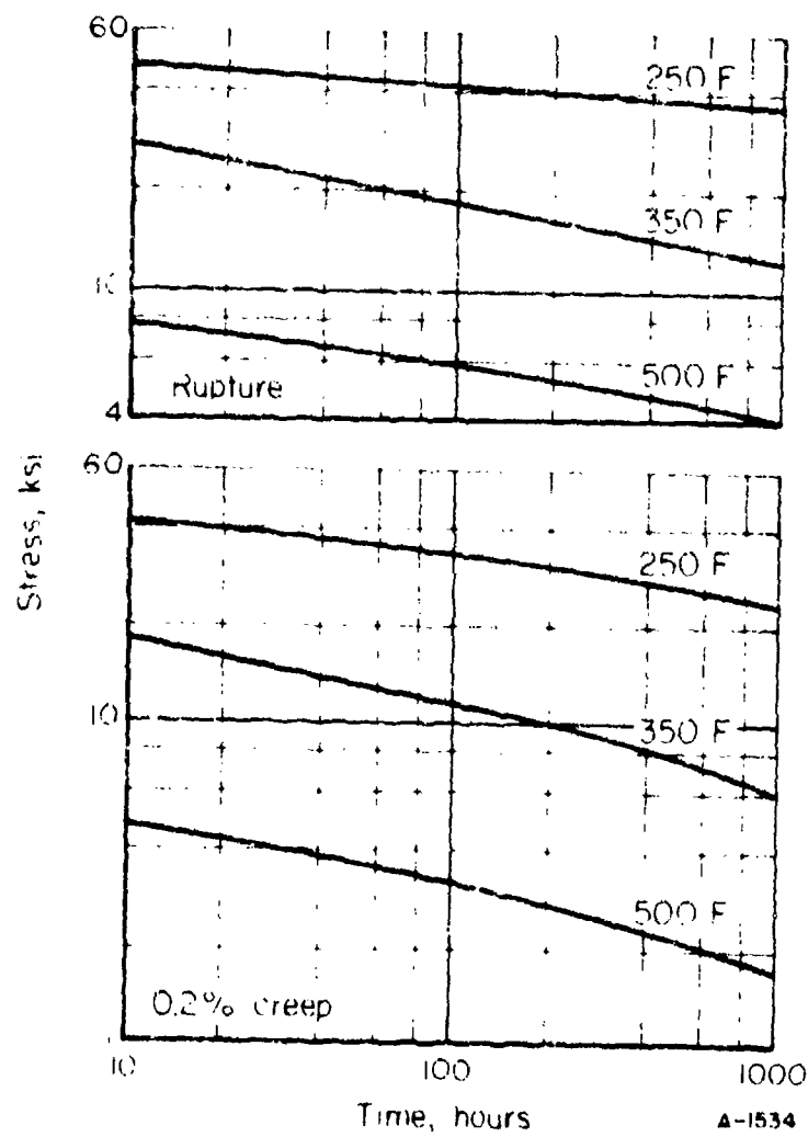
FIGURE 1. STRESS-TIME AND PLASTIC DEFORMATION CURVES FOR A-1534 ALLOY AT 250 F, 350 F, AND 500 F.
