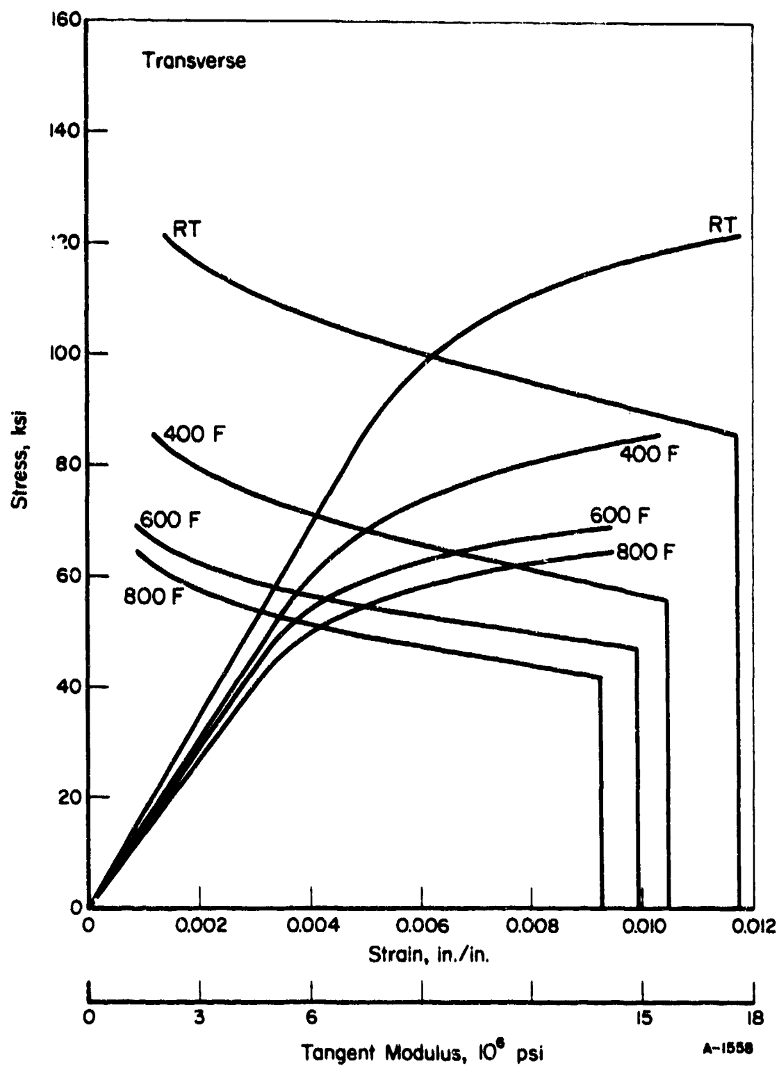
FIGURE 55. TYPICAL COMPRESSIVE STRESS-STRAIN AND TANGENT-MODULUS CURVES AT TEMPERATURE FOR ANNEALED Ti-6Al-2Cu-1Ta-1Mo ALLOY PLATE (TRANSVERSE)
