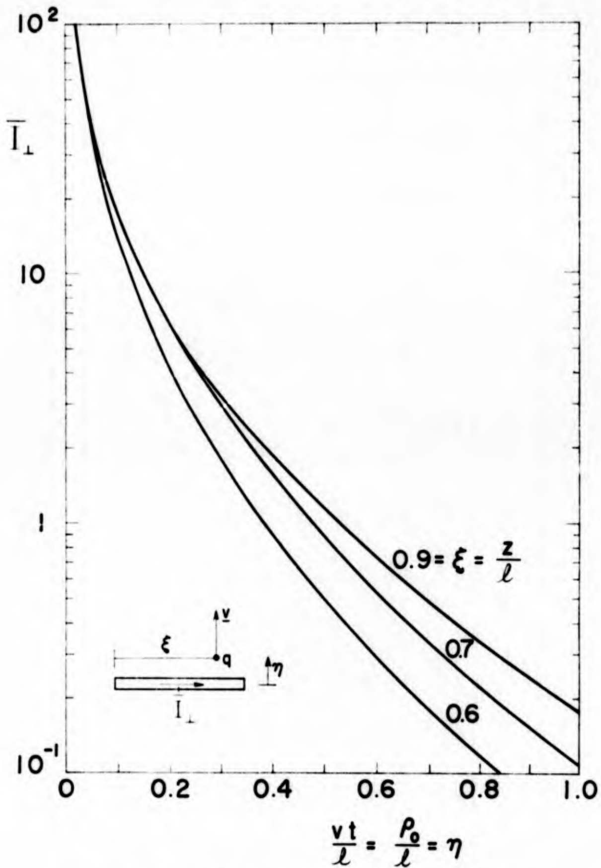
Figure 5. Normalized induced current for perpendicular motion.
