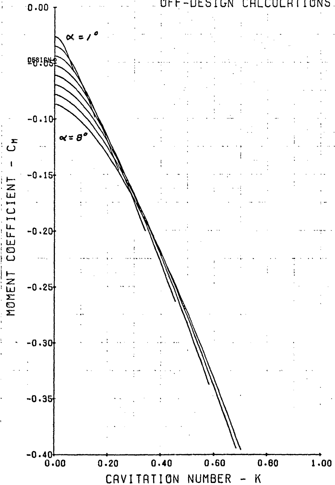
FIGURE-44 MOMENT COEFFICIENT VERSUS CAVITATION NUMBER. FIRST DESIGN PROCEDURE.
