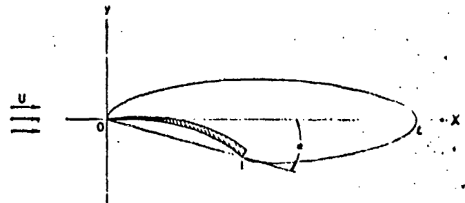
Fig. 1 Schematic diagram of cavity flow past a hydrofoil
