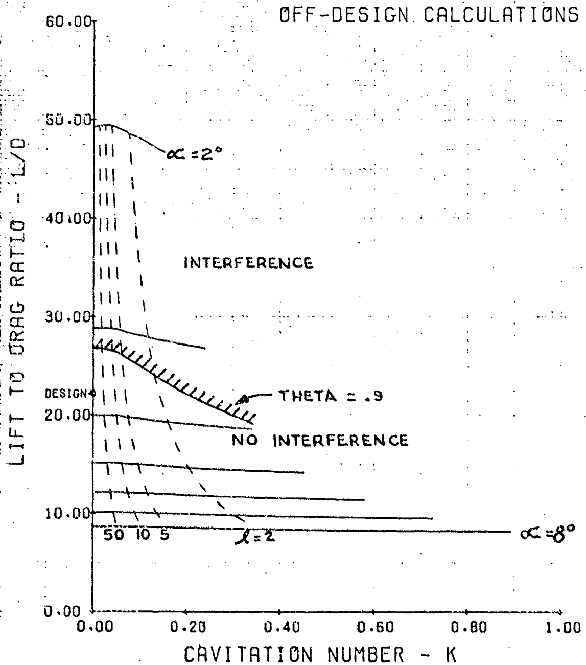
FIGURE-41 LIFT TO DRAG RATIO VERSUS CAVITATION NUMBER.
