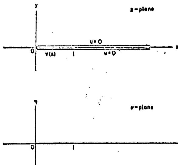
Fig. 2 Boundary conditions in the physical plane ( z -plane) and corresponding boundaries in the transformed plane ( v -plane) for zero cavitation number
