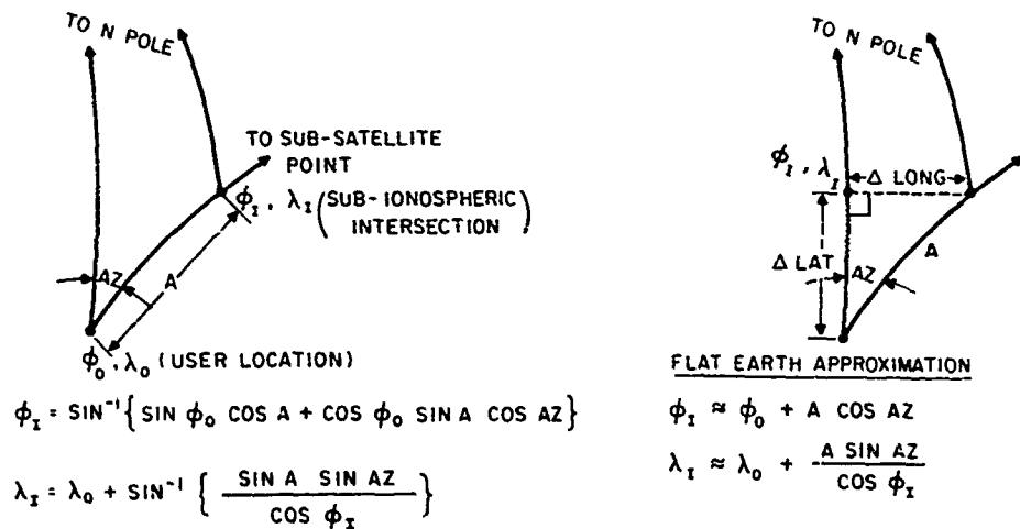
Figure 3. Approximations to Finding Sub-Ionospheric Coordinates
