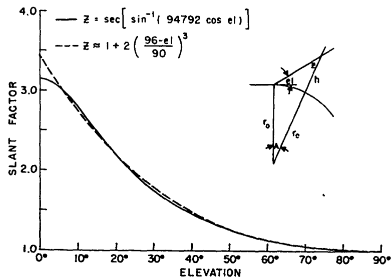
Figure 5. Approximation to Slant Factor, Z
