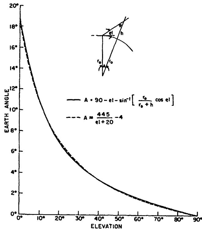
Figure 2. Approximation to Earth Angle, A
