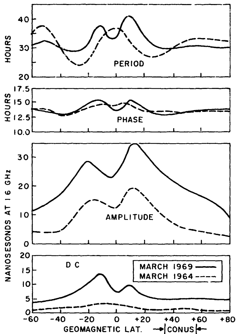
Figure 7. Cosine Model Coefficients (Bent Model) vs Geomagnetic Latitude for the Month of March for the Solar Minimum Year 1964 and the Solar Maximum Year 1969
