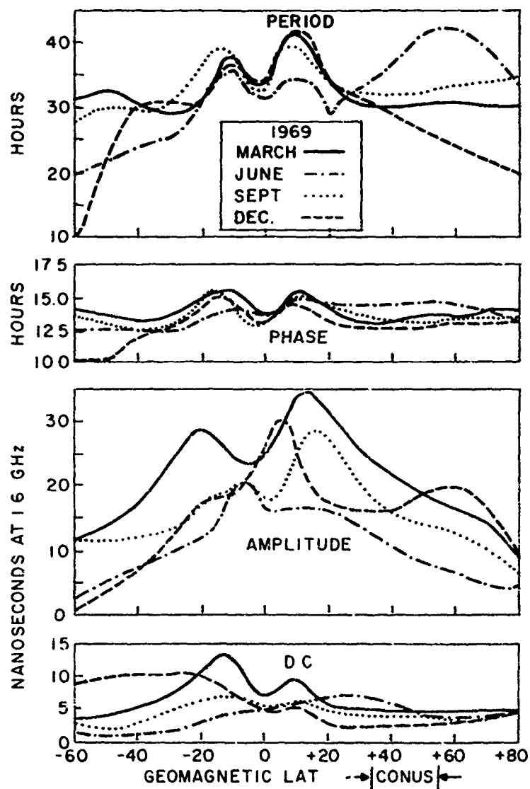
Figure 6. Cosine Model Coefficients (Bent Model) vs Geomagnetic Latitude for Four Seasons, 1969
