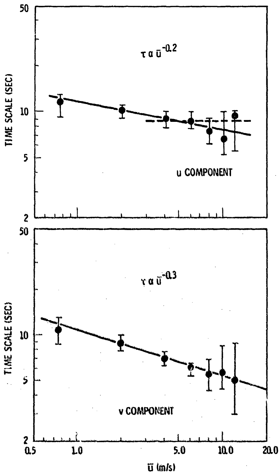
FIGURE 45. Variation of the horizontal component time scales with wind speed at the height of measurement.
