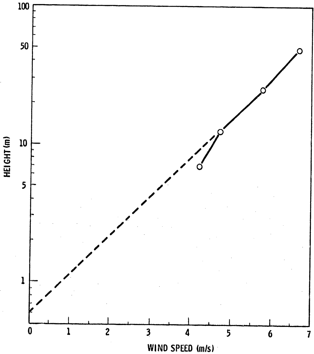
FIGURE 21. Composite wind profile for the extended tests at Lake Union.
