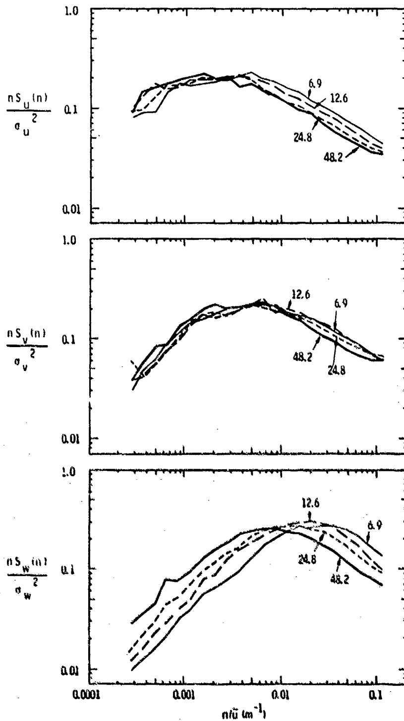
FIGURE 22. Composite spectra for the Lake Union intensive measurement data.
