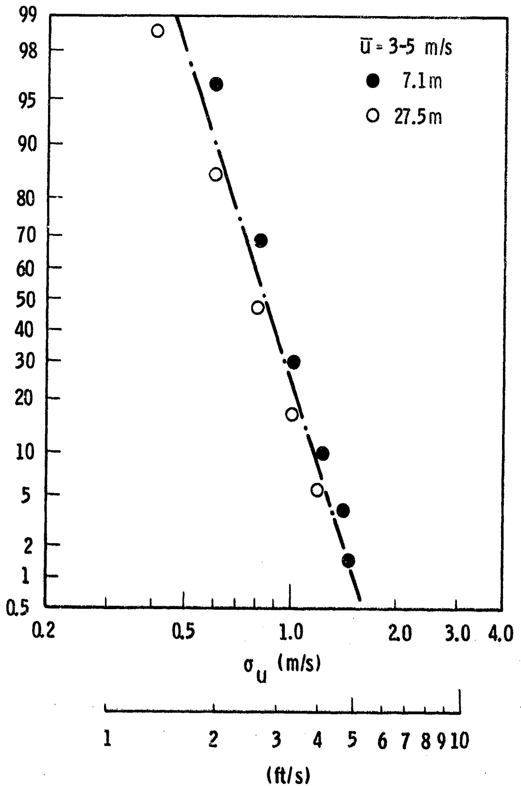
FIGURE 39. Frequency distribution of longitudinal rms gust velocities observed at SEA-TAC during westerly winds between 3 and 5 m/s.
