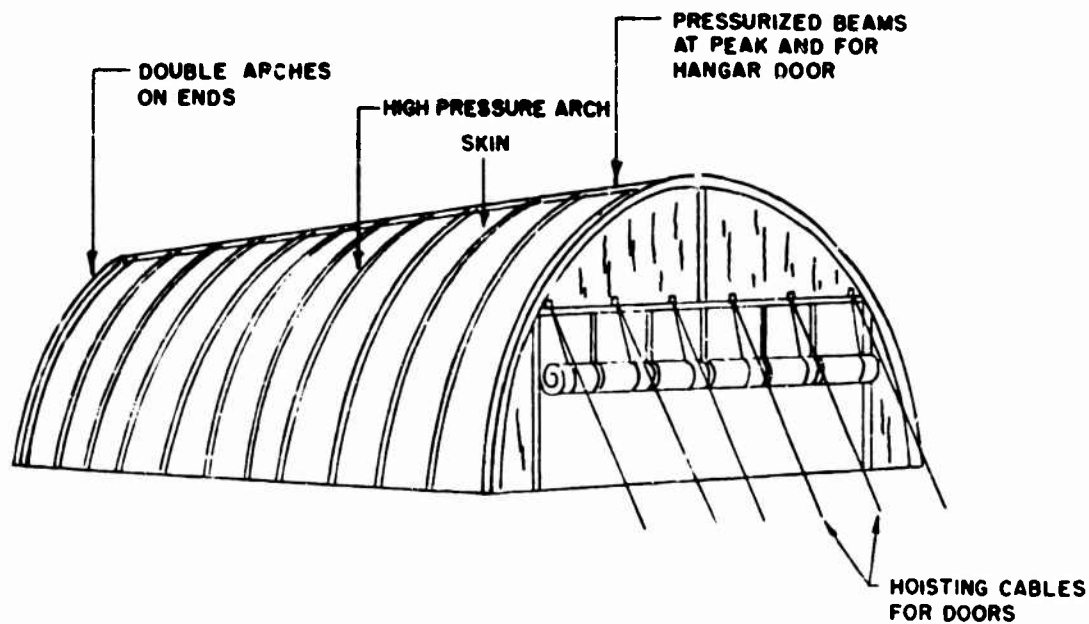
FIG. 3 PRESSURIZED RIB TENT CONCEPT FOR THE RMH
