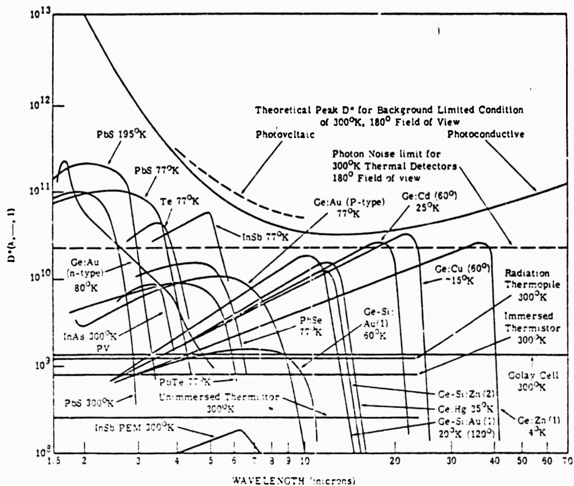
Figure 4-6. Characteristic Responses of Various Infrared Detectors
