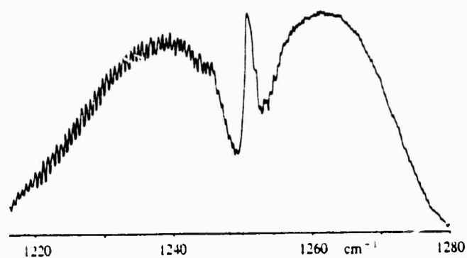
Figure 2-7e. The Parallel Stretching Vibration, Centered at 1251 \text{ cm}^{-1} , of the Symmetric Top Molecule Methyl Iodide, \text{CH}_3\text{I} , Showing the Typical PQR Contour
