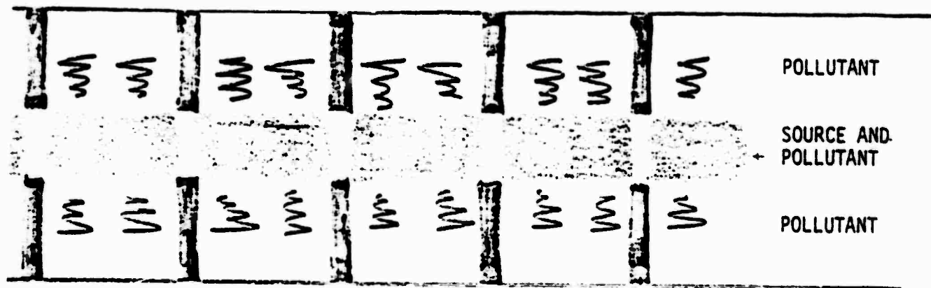
Figure 3-31. Spectra Observed with Spectrograph Slit Laid Across Sun's Glitter into Regions of Little Reflection from Earth's Surface
