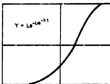
GOMPERTZ CURVE
