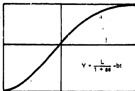
PEARL CURVE
