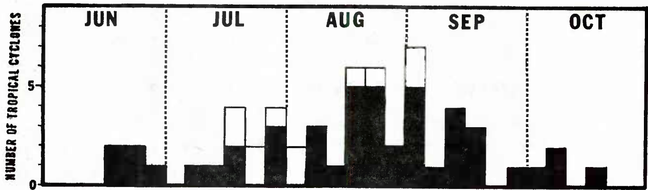
Figure 25. Frequency distribution of the number of tropical cyclones that passed within 180 n mi of Pusan/Chinhae. Subtotals are based on 5-day periods for tropical cyclones that occurred during 1947-1973. Shaded area indicates the number of recurring tropical cyclones per 5-day period.
