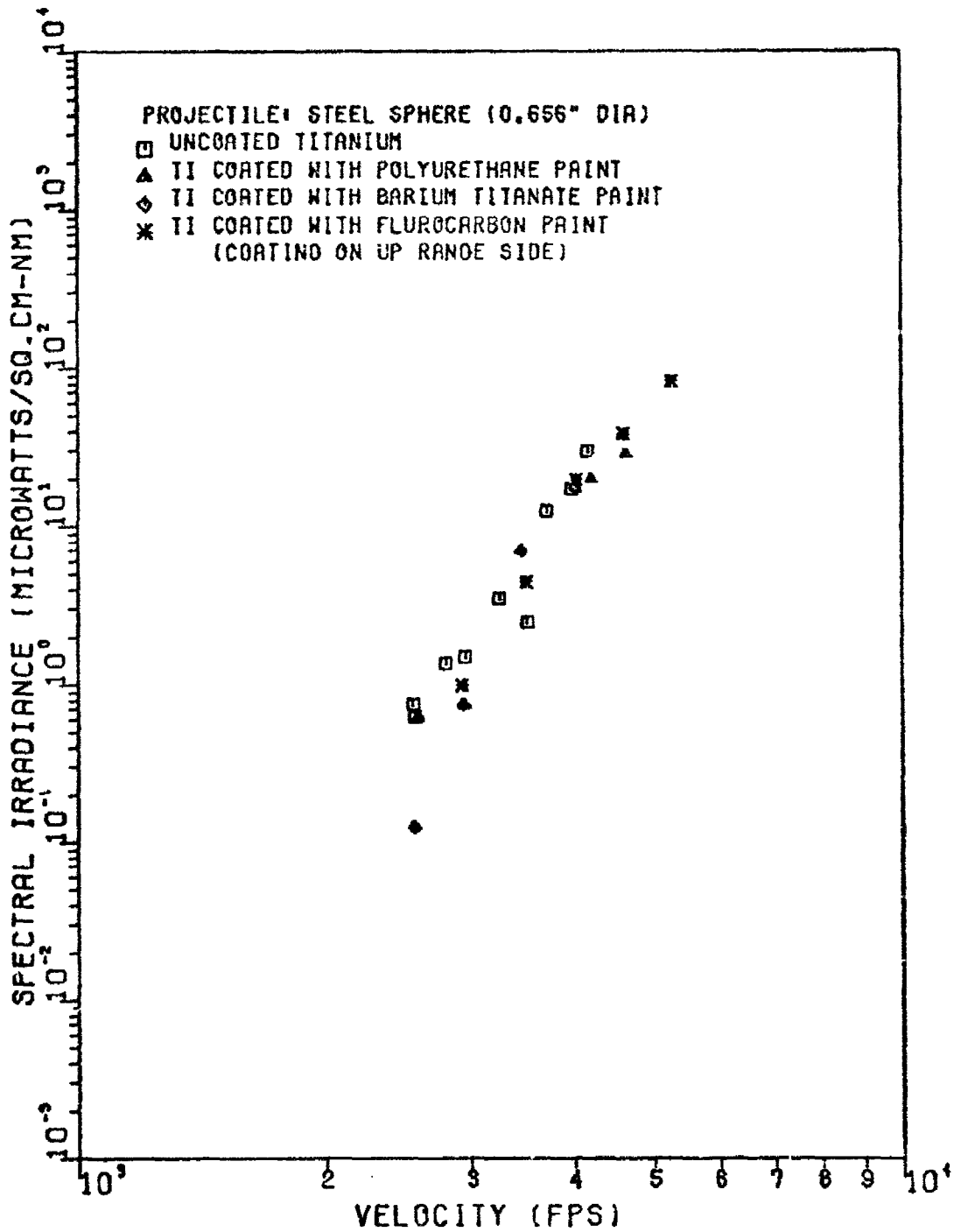
Figure 20. First Maxima of Spectral Irradiance at 9025A as a Function of Velocity
