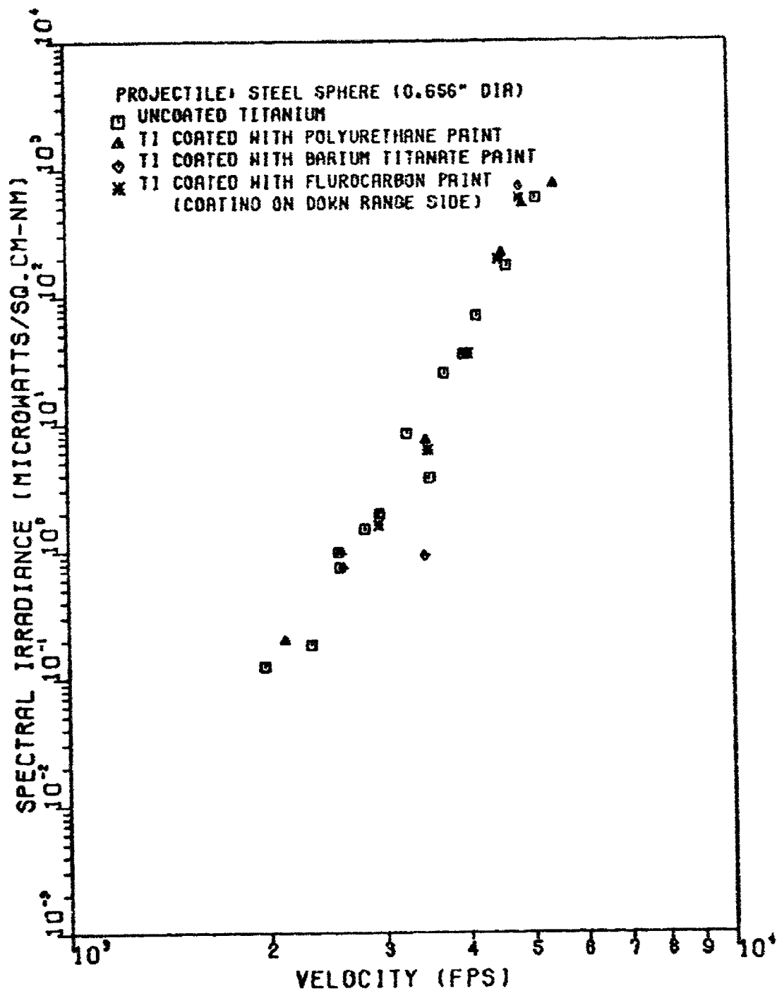
Figure 30. Second Maxima of Spectral Irradiance at 9025A as a Function of Velocity
