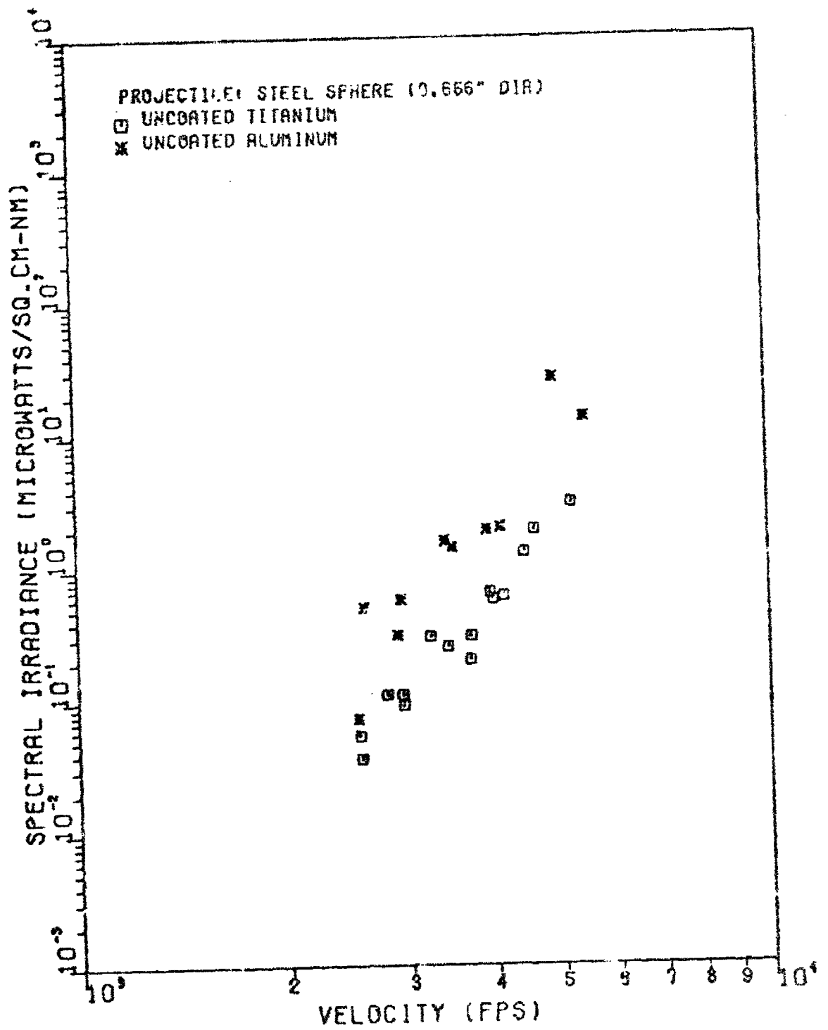
Figure 7. First Maxima of Spectral Irradiance at 4008A as a Function of Velocity
