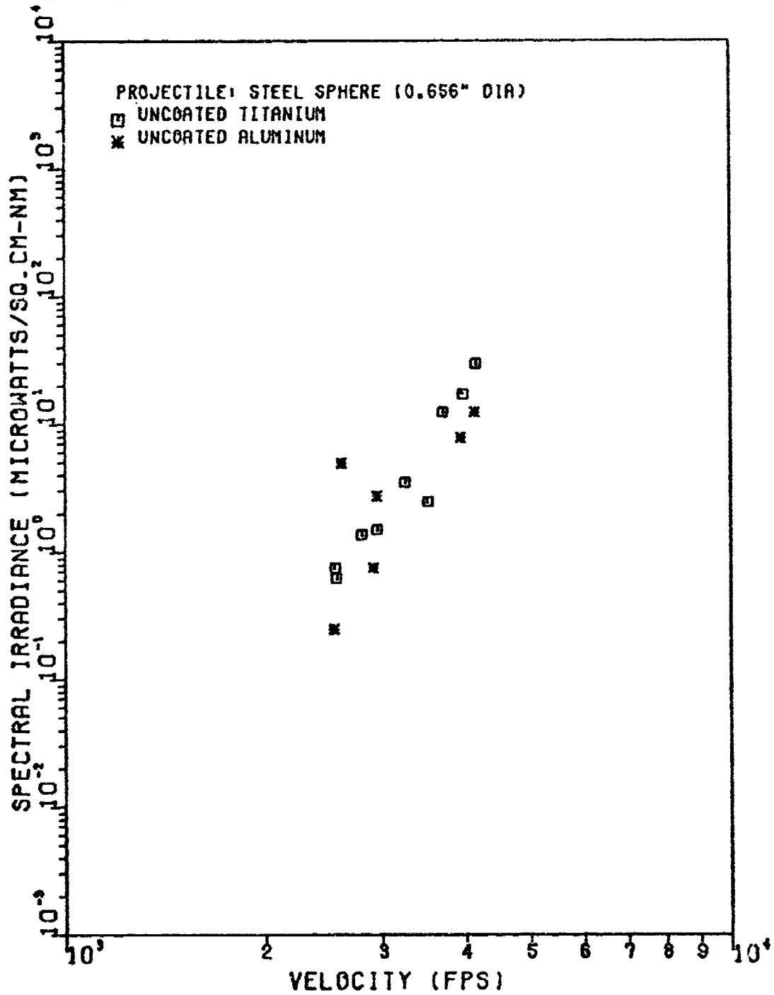
Figure 11. First Maxima of Spectral Irradiance at 9025A as a Function of Velocity
