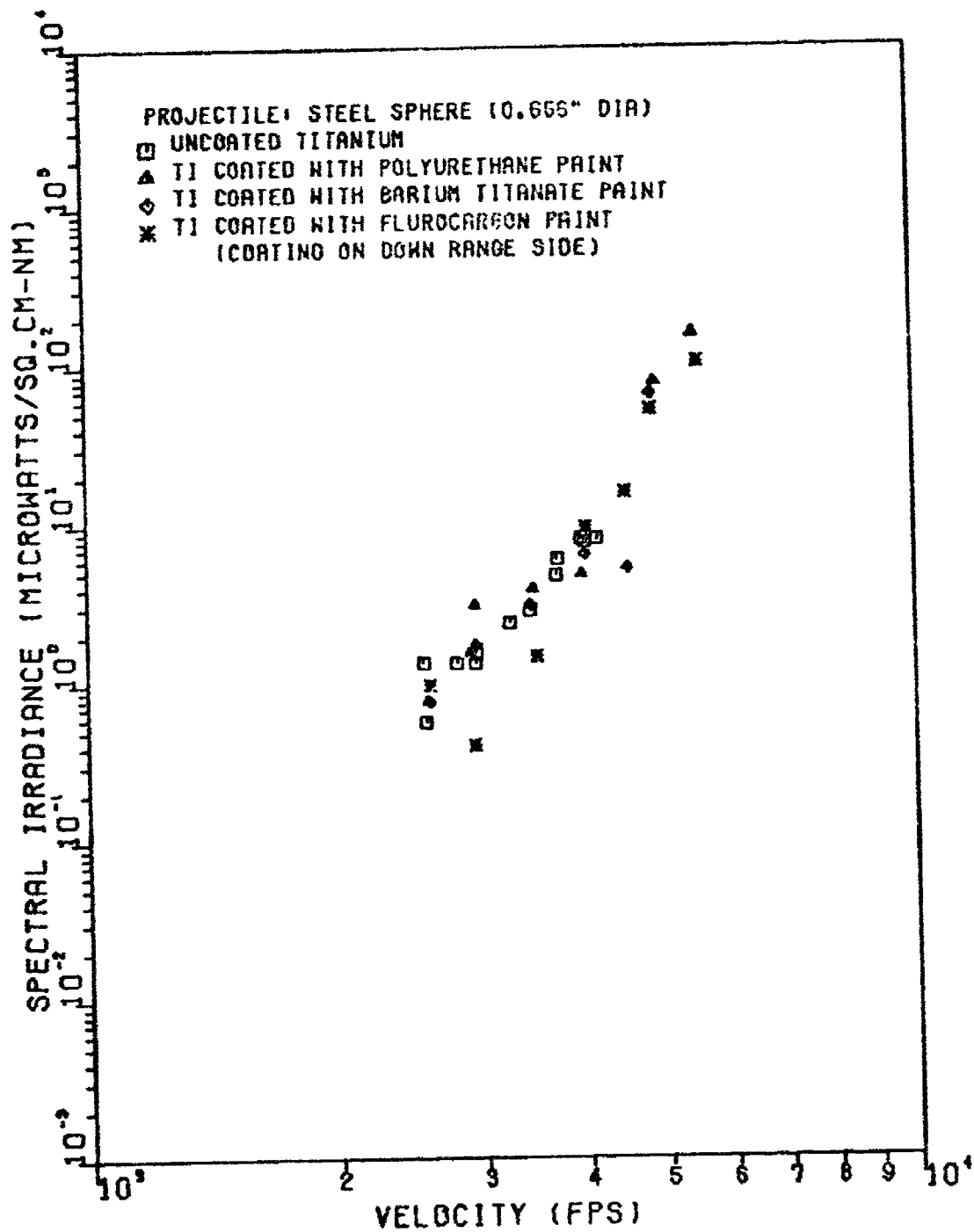
Figure 27. First Maxima of Spectral Irradiance at 7010A as a Function of Velocity
