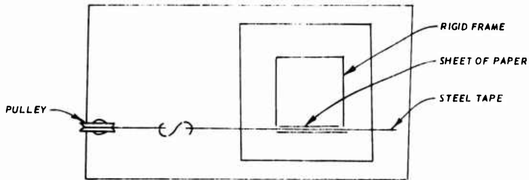
Figure 2. Terzaghi apparatus for determining earth pressure at rest
