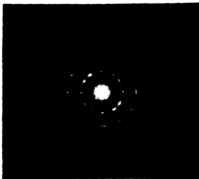
Figure 18. Electron diffraction patterns of InSb RF sputter deposited on cleaved NaI substrates (a) with no externally applied substrate bias and (b) with an applied bias of -25 V.
