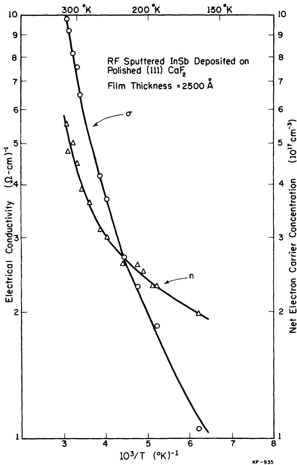
Figure 16. The temperature dependence of the net carrier concentration and electrical conductivity of a 2500 Å thick InSb film RF sputter deposited on p-a \text{CaF}_2 at 400°C.
