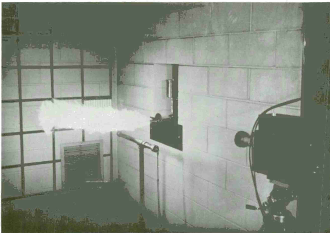
FIGURE A-2. PHOTOGRAPH OF A MIST FLASHBACK TEST WITH NEAT JP-8
