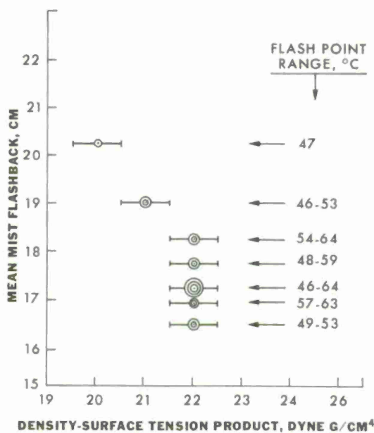
FIGURE A-3. MIST FLASHBACK PROPERTIES OF VARIOUS JP-8 AND JET A FUELS
