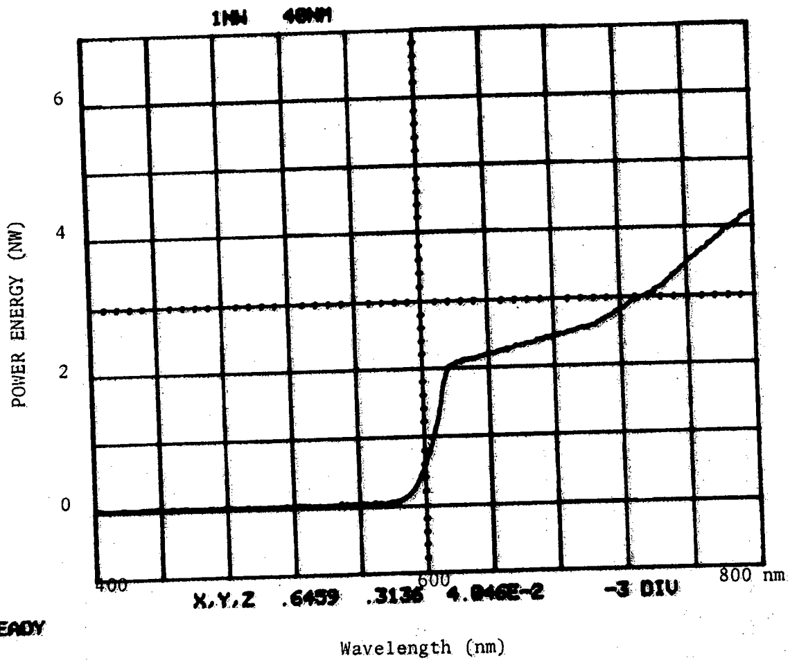
FIGURE 13. Spectral Transmittance for Navy Dark Adaptation Goggles
