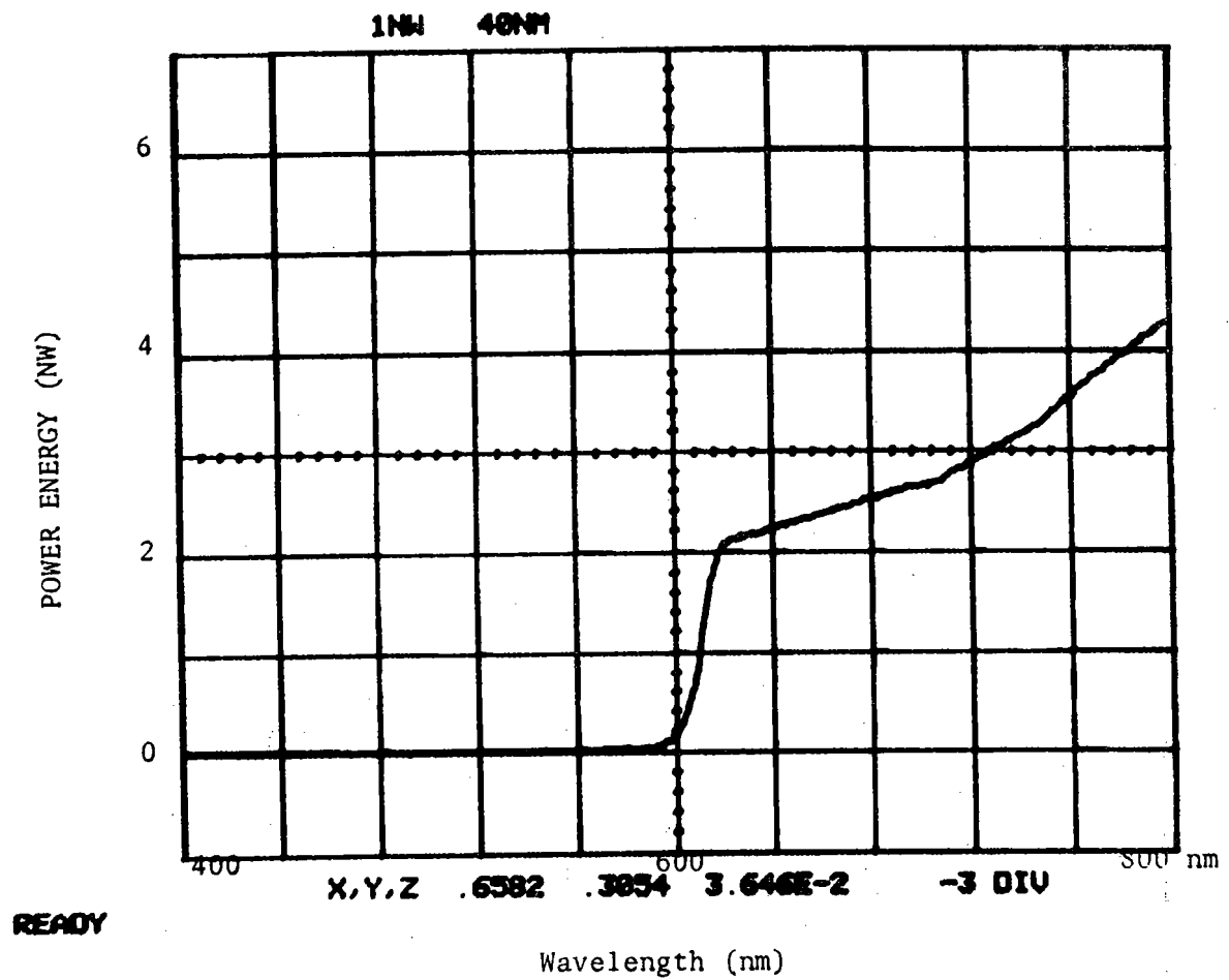
FIGURE 14. Spectral Transmittance for Fluoroscopy Dark Adaptation Goggles
