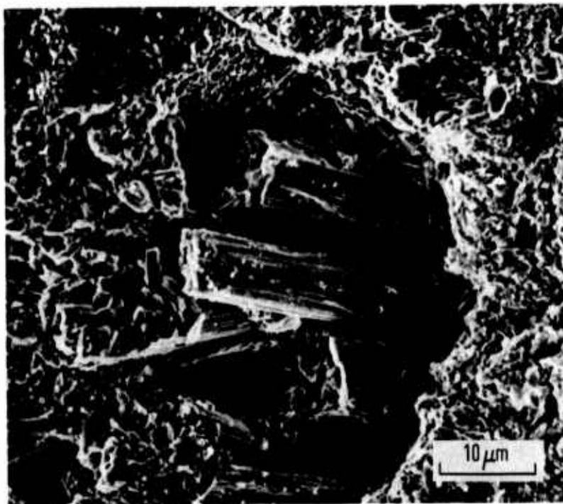
Figure 1. Pyrocarb 903 Backface
