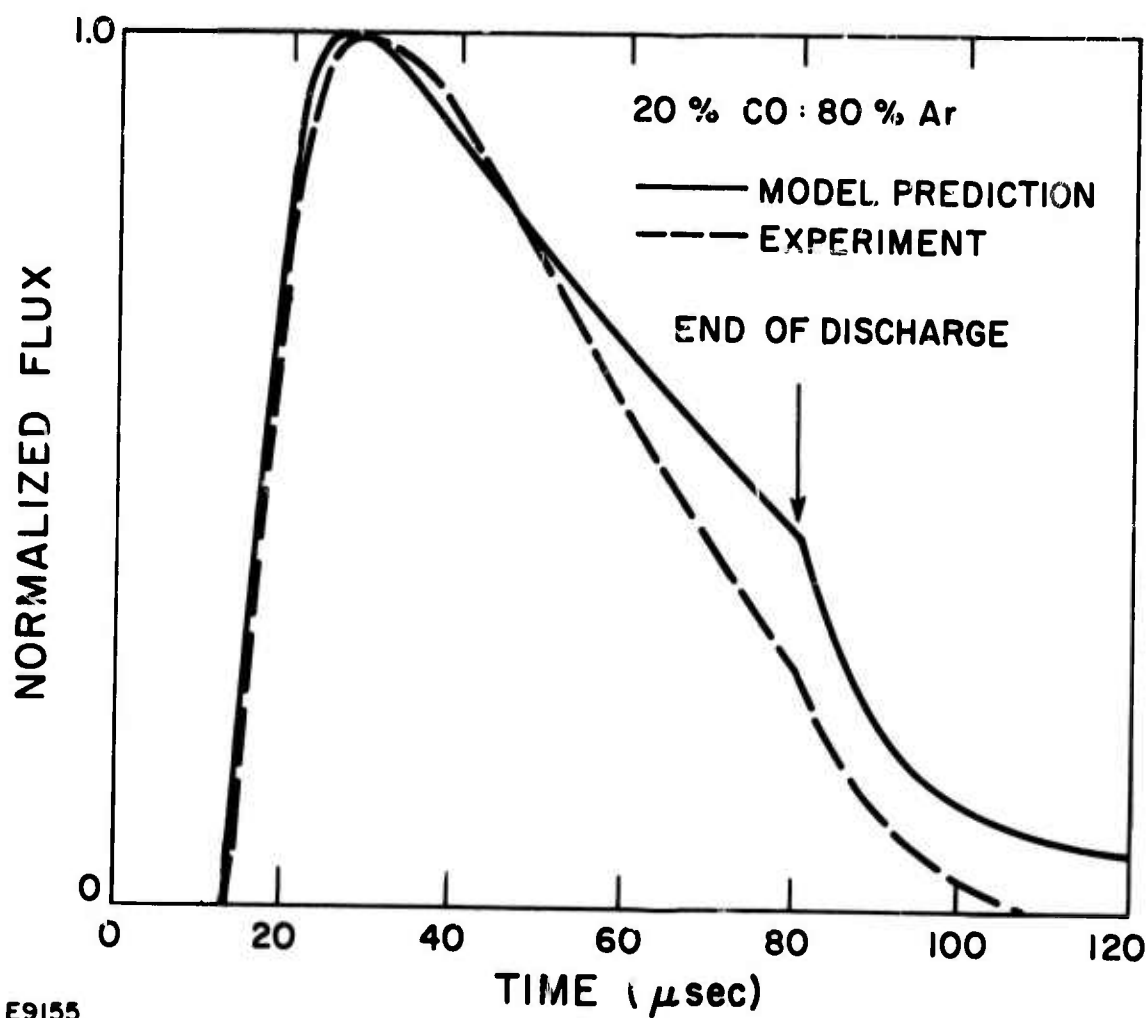
E9155 Fig. 3 Comparison of the Normalized Experimental and Predicted Temporal Behavior of the Laser Output Pulse for a 20% CO and 80% Ar Mixture
