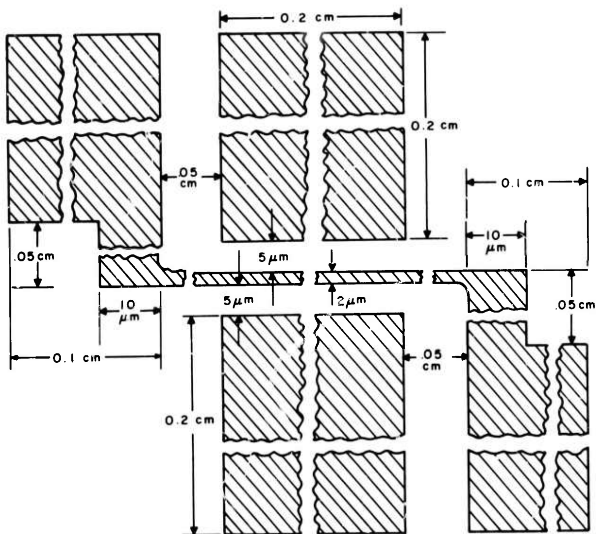
Figure 8. Dimensional drawing of electrodes for electro-optic modulation of stripe guide couplers.
