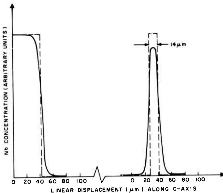
Figure 5. Distribution of Nb about the edge of a planar waveguide region (left) and a stripe of 14-μm nominal width (right). The stripe pattern ran perpendicular to the a-axis and was formed on a substrate cut perpendicular to the x-axis (i.e., an "x-plate"). The diffusion conditions (1100°C for 6 hours) were chosen to yield a 1-μm diffusion depth. The dotted lines show the inferred position of the initial metallic pattern.
