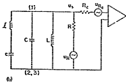
FIG. 3. Electrical equivalent representations of electrons in the Penning trap structure. (a) Electrical representations of electrons in the Penning trap and electrical equivalent representation. (b) Electrical equivalent representation of electrons, Penning trap, and external circuitry having noise voltages associated with trap resistance R and Heitlinger's transistor input noise resistor R_n .
