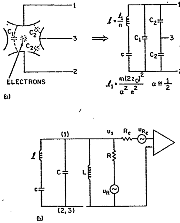
Fig. 7. Electrical equivalent representations of electrons in the Penning trap structure. (a) Pictorial representation of electrons in the Penning trap and electrical equivalent representation. (b) Electrical equivalent representation of electrons (l, c), Penning trap, and external circuit (L, C) showing noise voltages associated with real resistance R and fictitious transistor input noise resistor $R_e$, from (Wineland & Dehmelt, 1975b)
