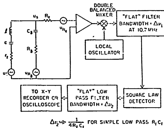
Fig. 8. Narrow frequency band model for electrons/ions (l, c, $r_z$) interacting with LC circuit ($C_0$, $R_0$) showing block diagram of detection electronics, from (Wineland & Dehmelt, 1975b).
