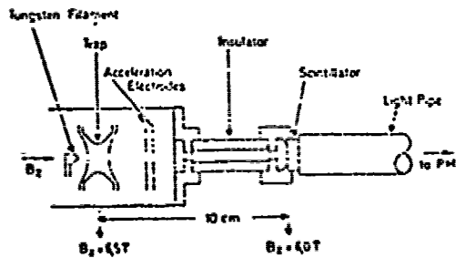
Fig. 1. Schematic diagram of electron trap and detection system.
