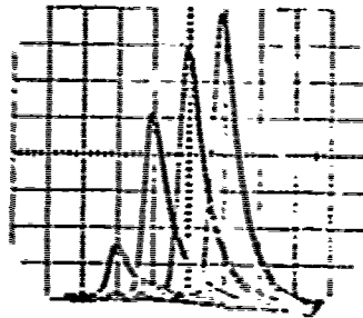
Oscilloscope presentation of the detection of ions by the resonance method. Peaks represent number of H + ions in the trap. The production is by photoionization of the simultaneously trapped H 2 + . The four peaks are for H + collection times of 50, 250, 450, and 650 msec. The largest represents 10% damping. Time base is 1 msec/division.
