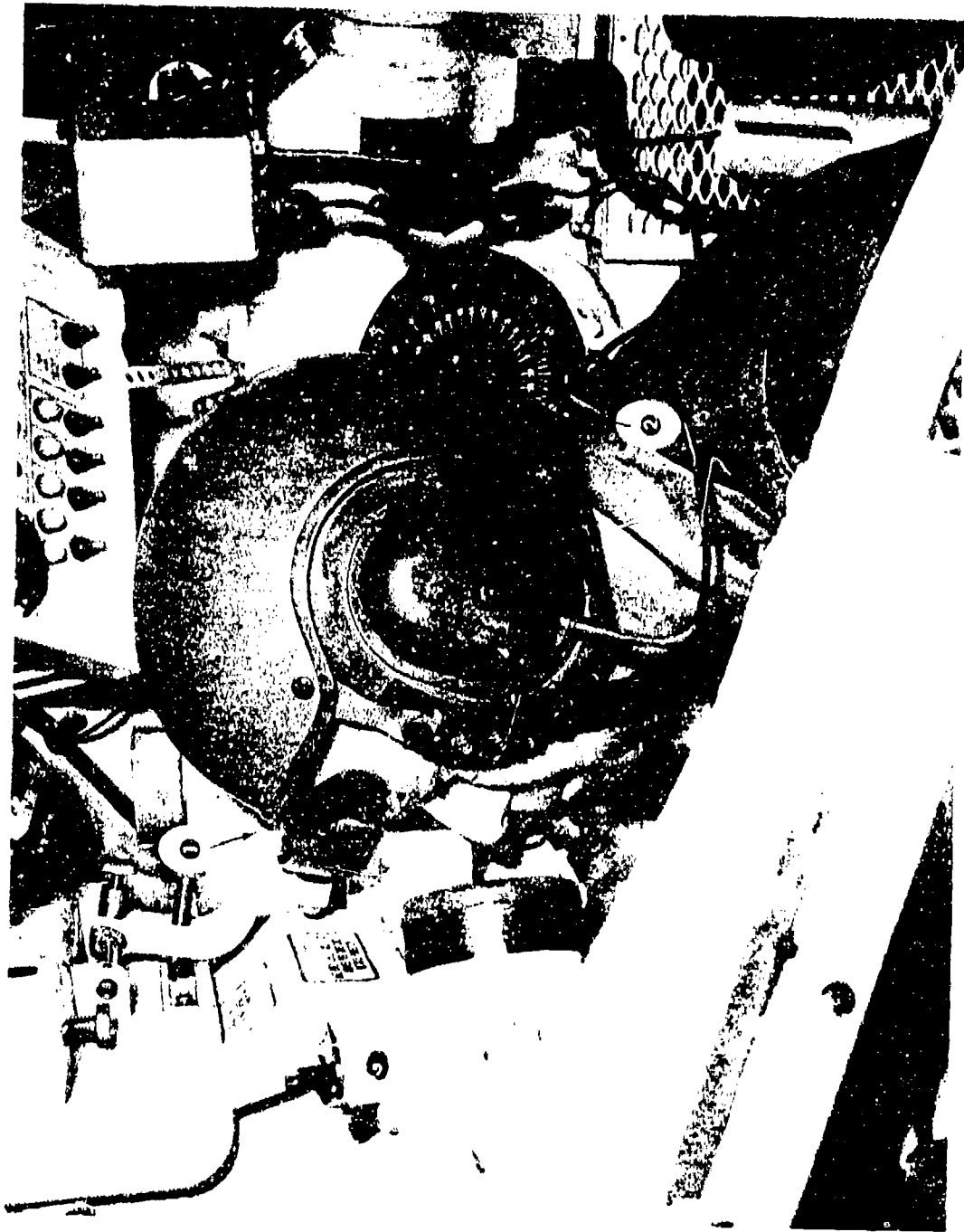
Fig. 30. M551 (Sheridan) gunner viewing with M144 periscope (night sight), full bar browpad, type 5, forehead against browpad, DH-132 helmet tilted back.
