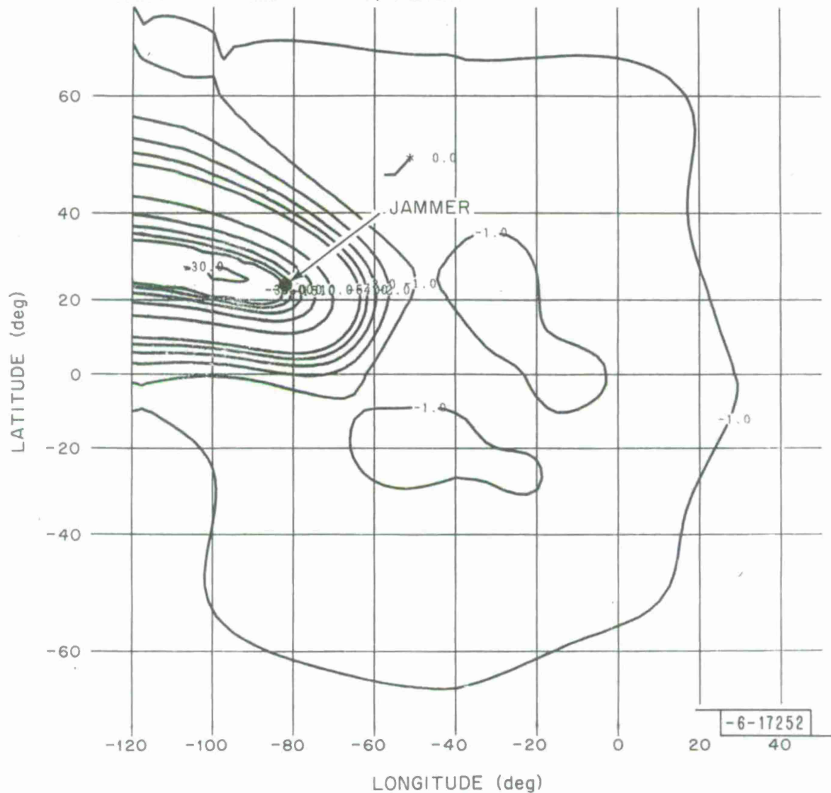
Fig. 30. Earth-coverage contour plot for the 28-inch lens/61-element cluster with feeds 62, 71 and 72 excited 180^\circ out-of-phase with relative power excitation -14.2 dB.
