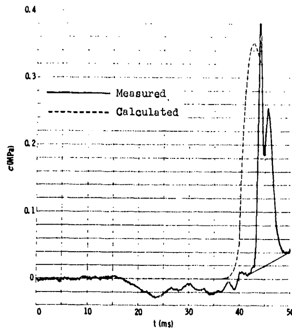
Figure V-14 Mean Stress History Measured at Z = 5.59 \text{ m} and K = 0.45 \text{ m} (Time of Impact = 2 ms).
