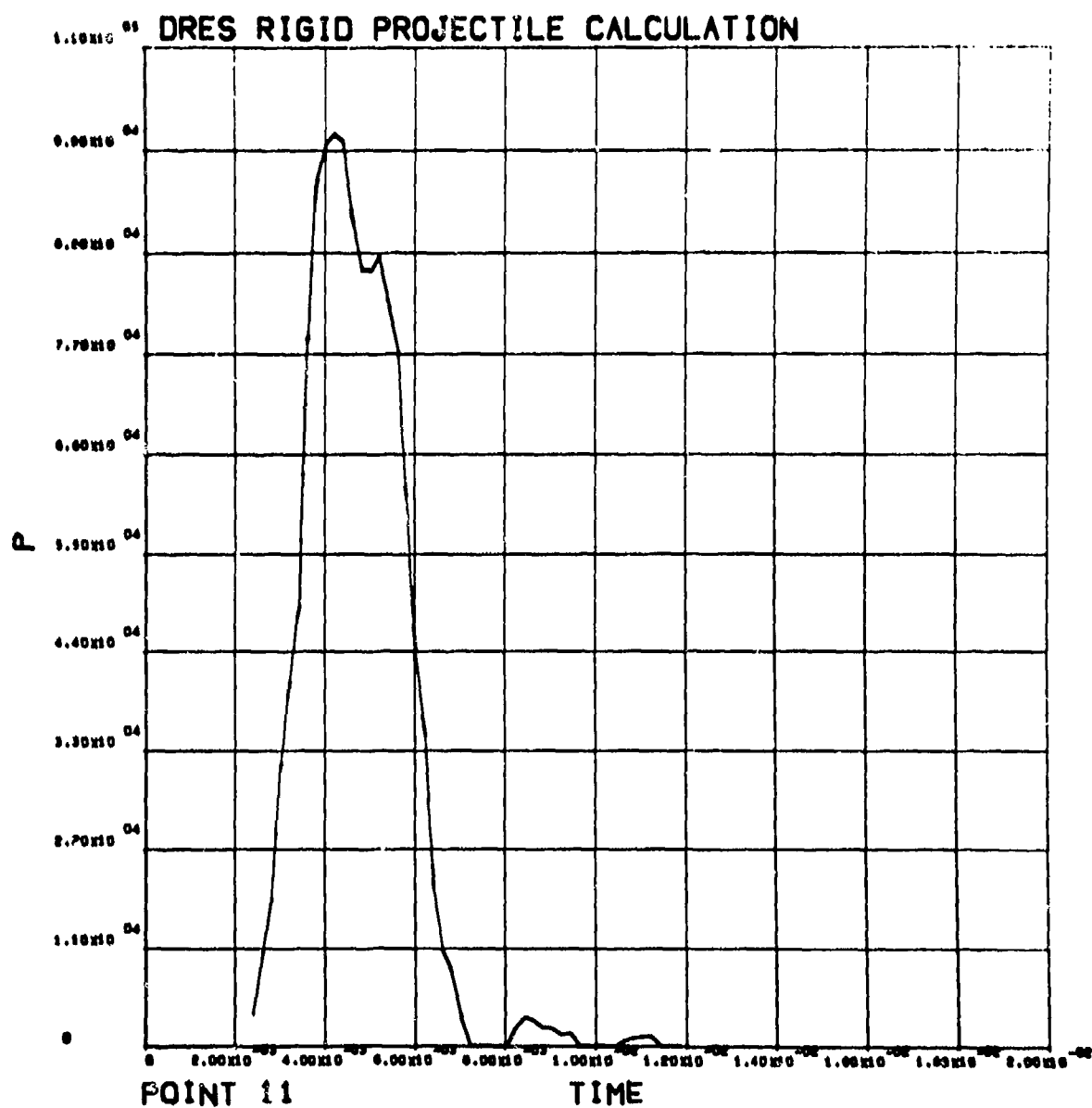
Figure A-63 Pressure (Pa) versus Time (s) for Particle at Point 11, Z = 0.1 m, R = 0.45 m.
