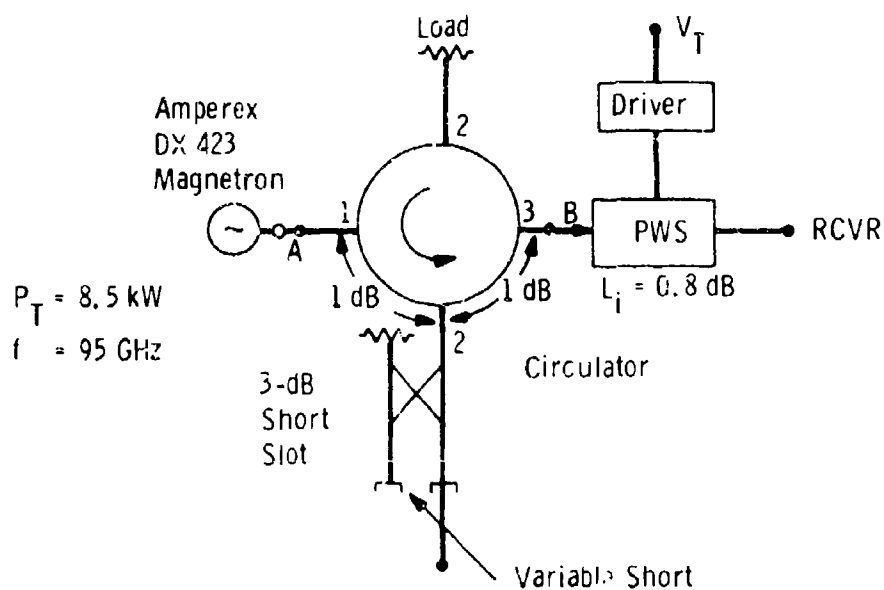
Circulator-Inline RP Duplexer Radar Configuration
