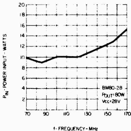
POWER INPUT vs FREQUENCY
