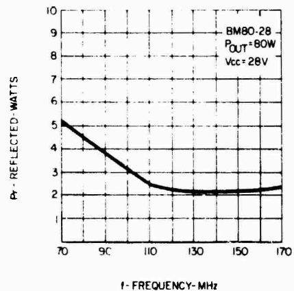
INPUT MATCH vs FREQUENCY
