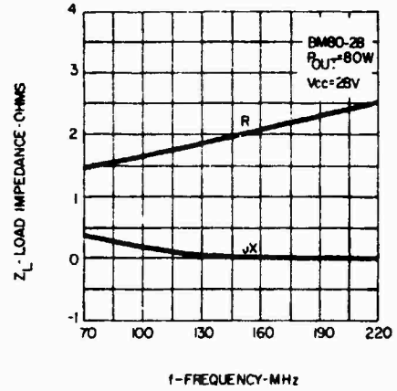
SERIES LOAD IMPEDANCE VERSUS FREQUENCY
