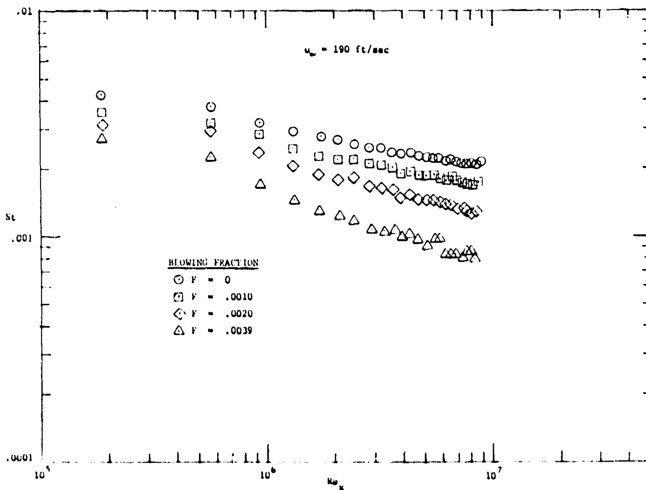
Fig. 3.15 Rough surface Stanton number versus x-Reynolds number at u_{\infty} = 190 \text{ fps}
