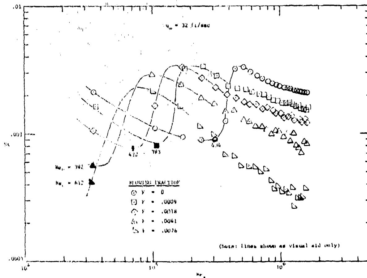
Fig. 3.9 Rough surface Stanton number versus x-Reynolds number at u_\infty = 32 fps
