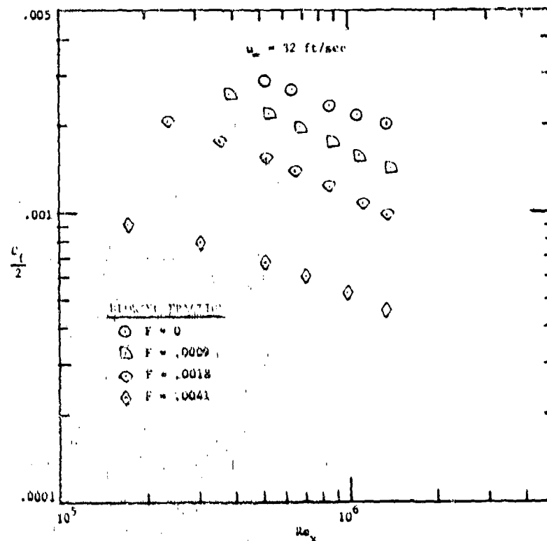
Fig. 3.8 Rough surface skin friction versus x-Reynolds number at u_\infty = 32 fps
