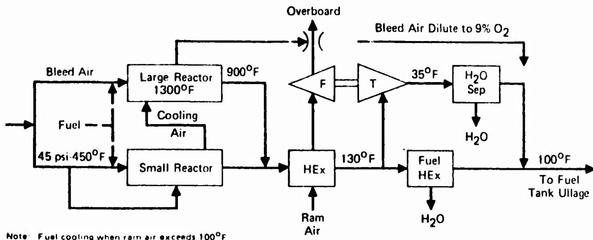
FIGURE 27 SORBENT-BASED INERTANT GENERATOR
