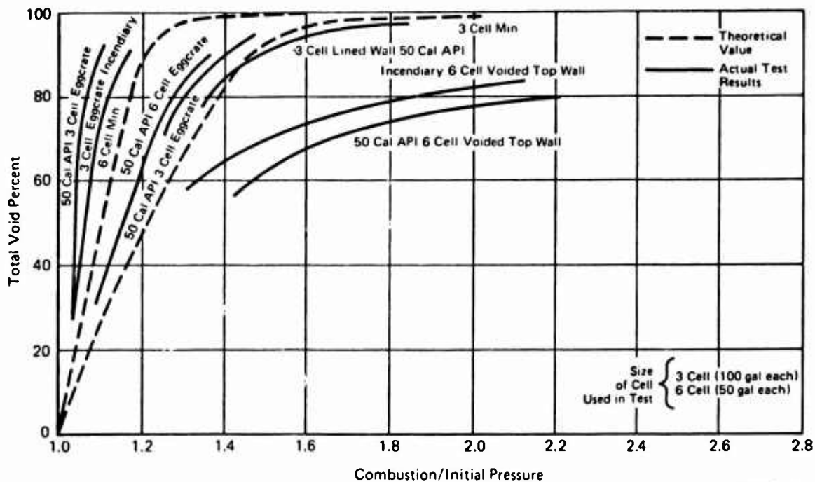
FIGURE 20 FUEL TANK GROSS VOIDED FOAM GUNFIRE AND INCENDIARY DATA
