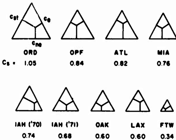
FIGURE 1. Relationship between c_{st} , c_e , and c_{ne} represented on the Stren triangle. The size of the triangle is proportional to C_s .
