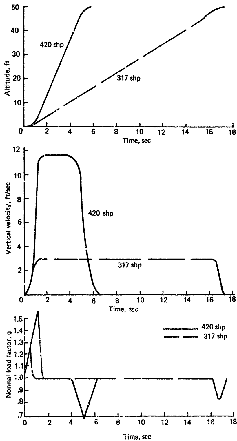
Figure 2. Bob-up from hover to 50 feet.
