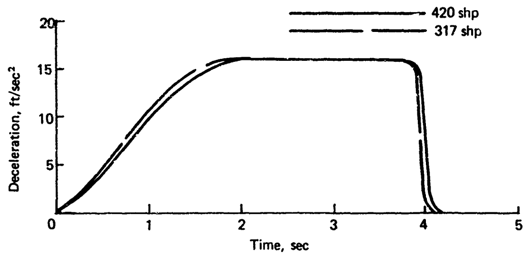
Figure 7. Longitudinal deceleration from 30 knots.
