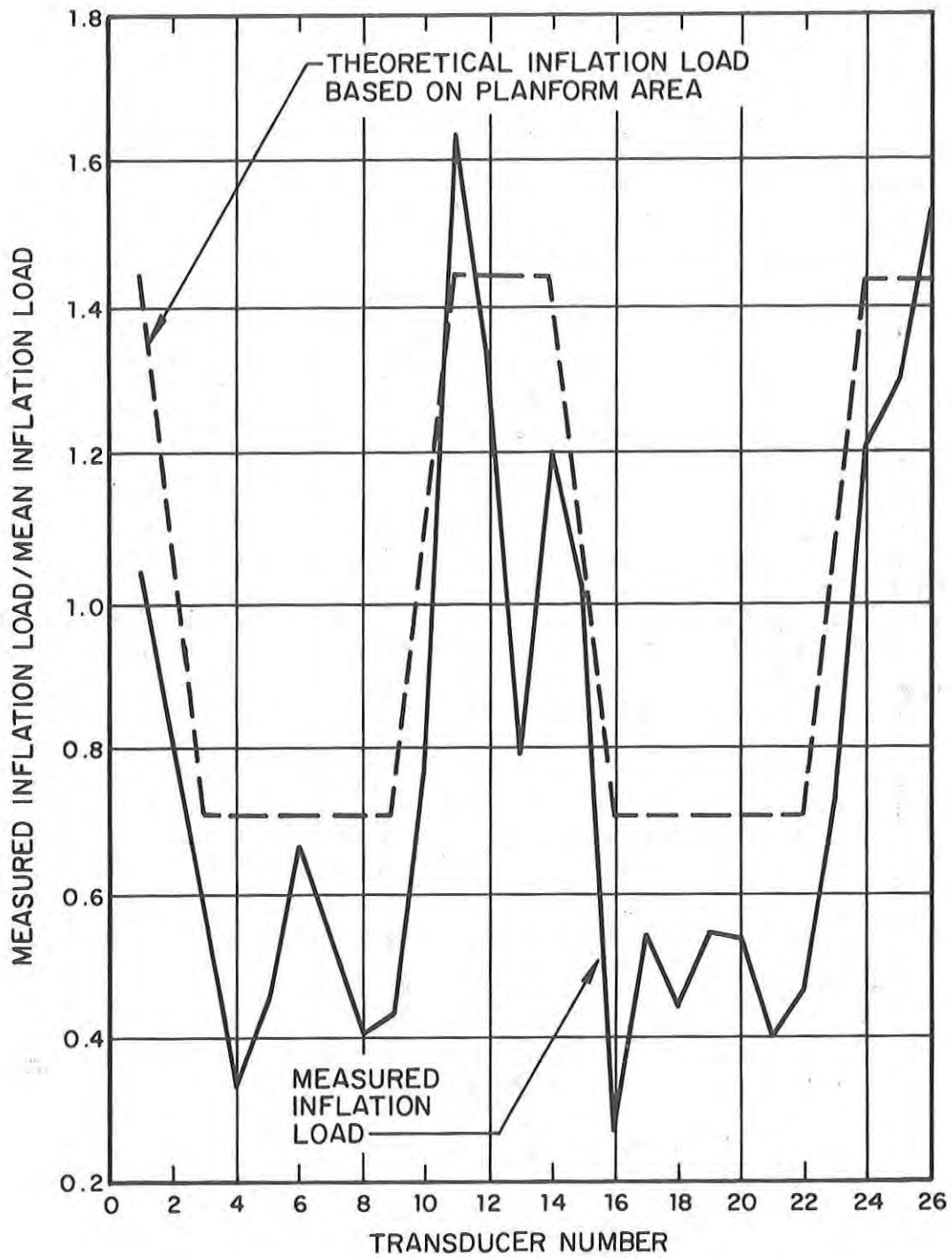
FIG. 20. INFLATION LOAD DISTRIBUTION.
