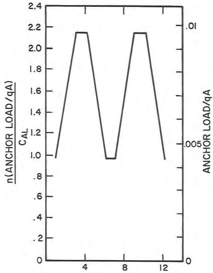
(a) ANCHOR LOAD
