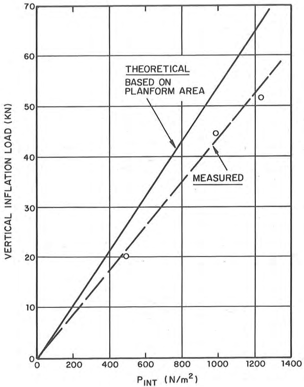
FIG. 19. VERTICAL INFLATION LOAD AS A FUNCTION OF INTERNAL PRESSURE.
