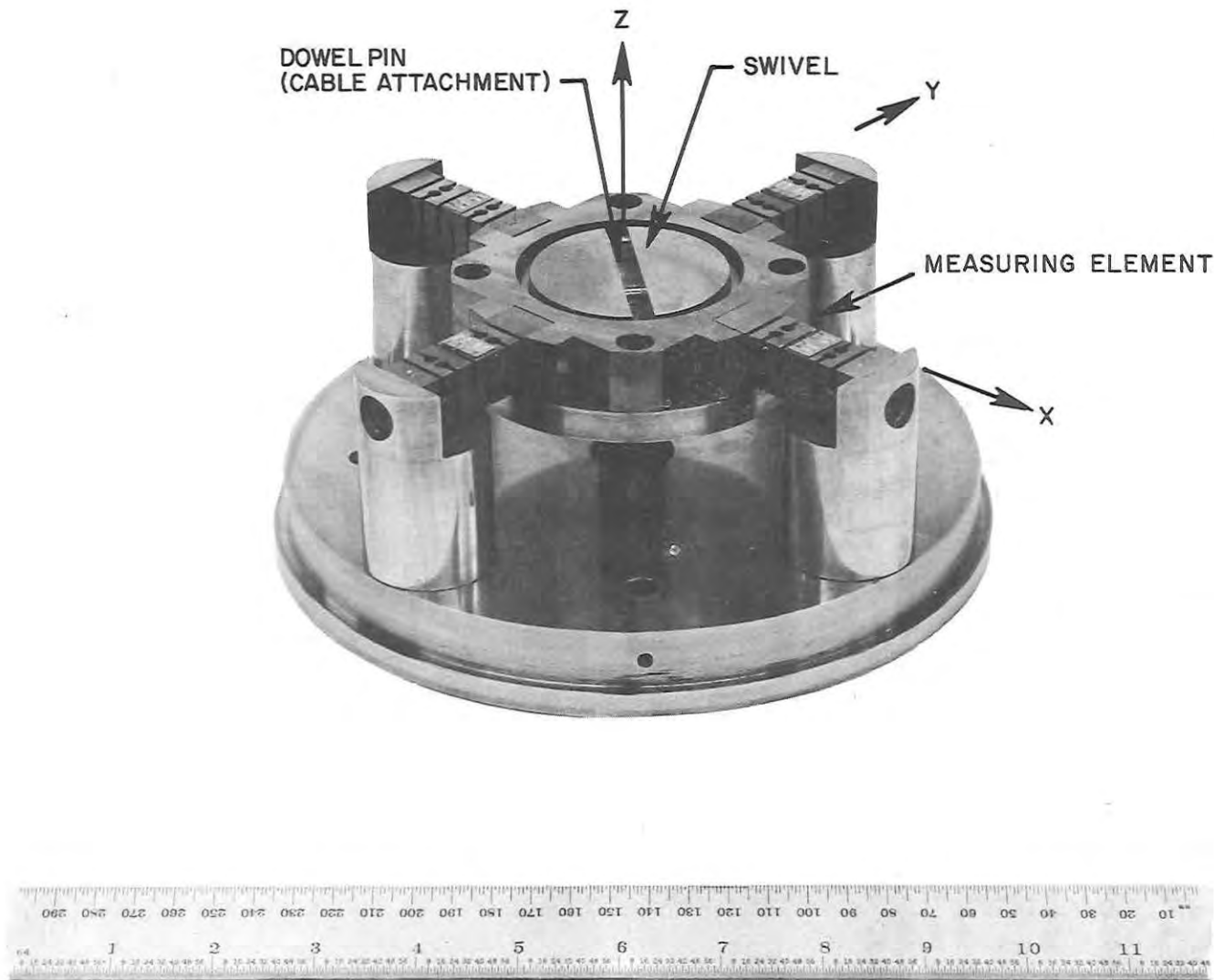
FIG. 8. THREE COMPONENT LOAD TRANSDUCER WITH COVER REMOVED.
