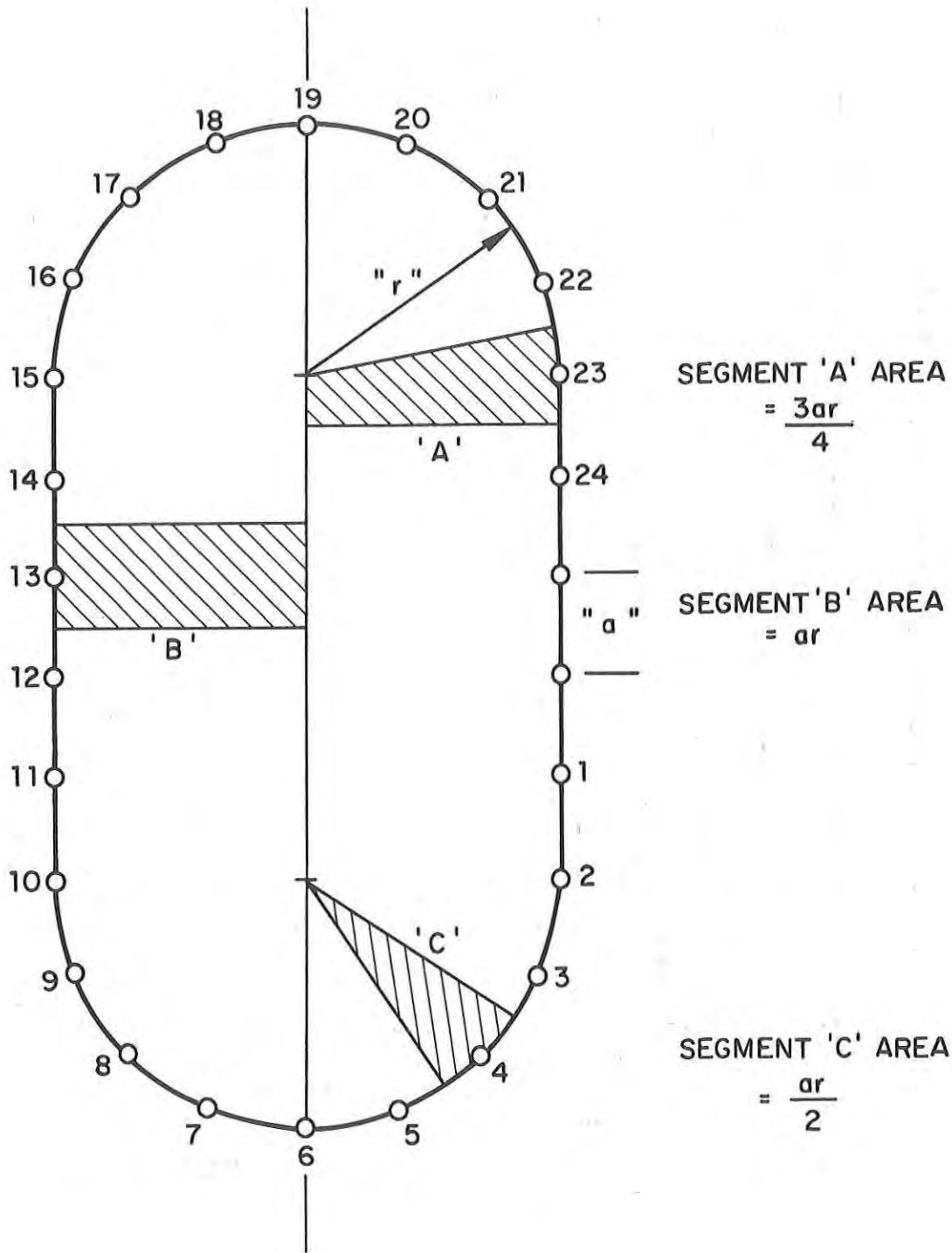
FIG. 21. PLANFORM AREA DISTRIBUTION FOR LOADING PROFILE.
