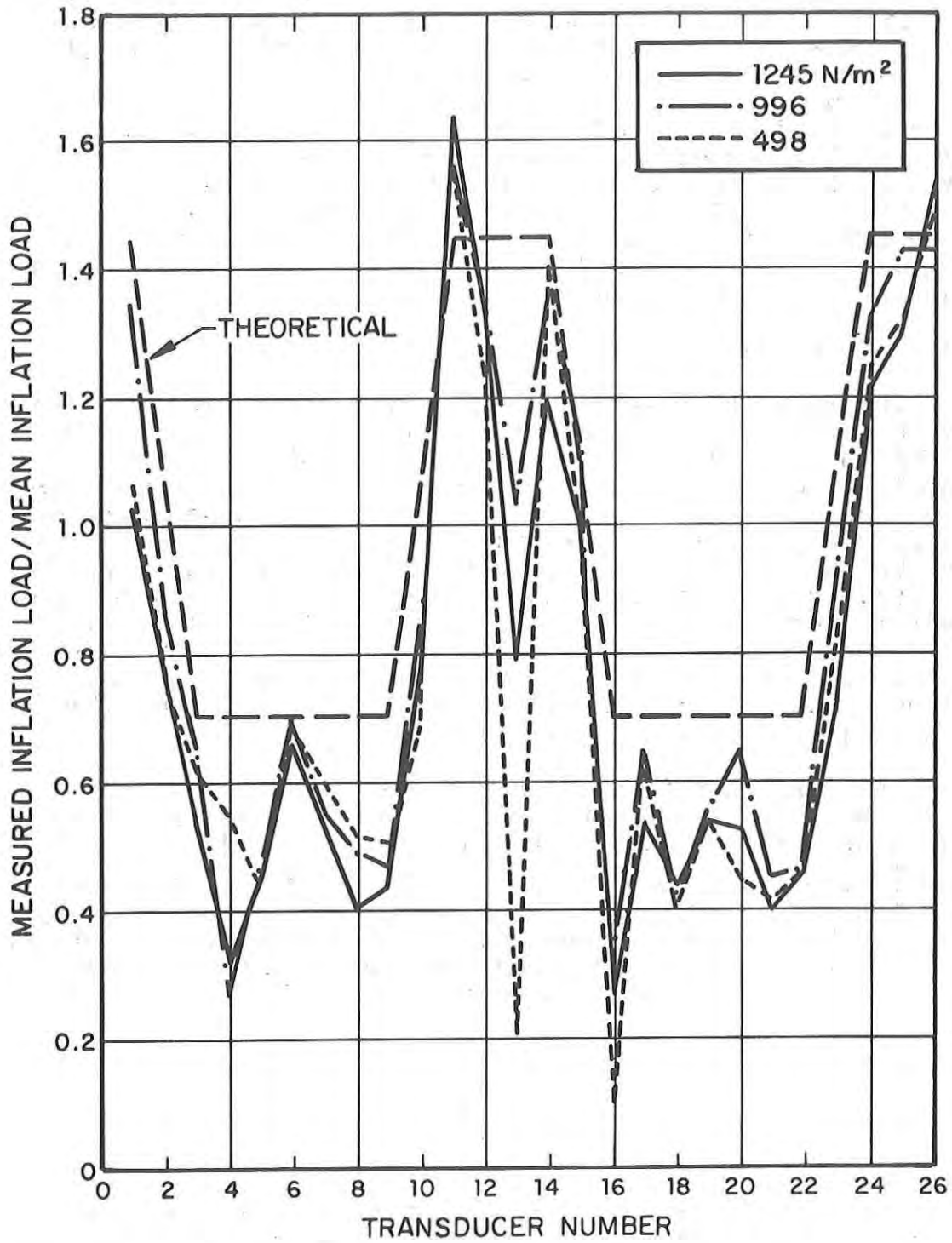
FIG. 22. SUMMARY OF INFLATION LOADS.
