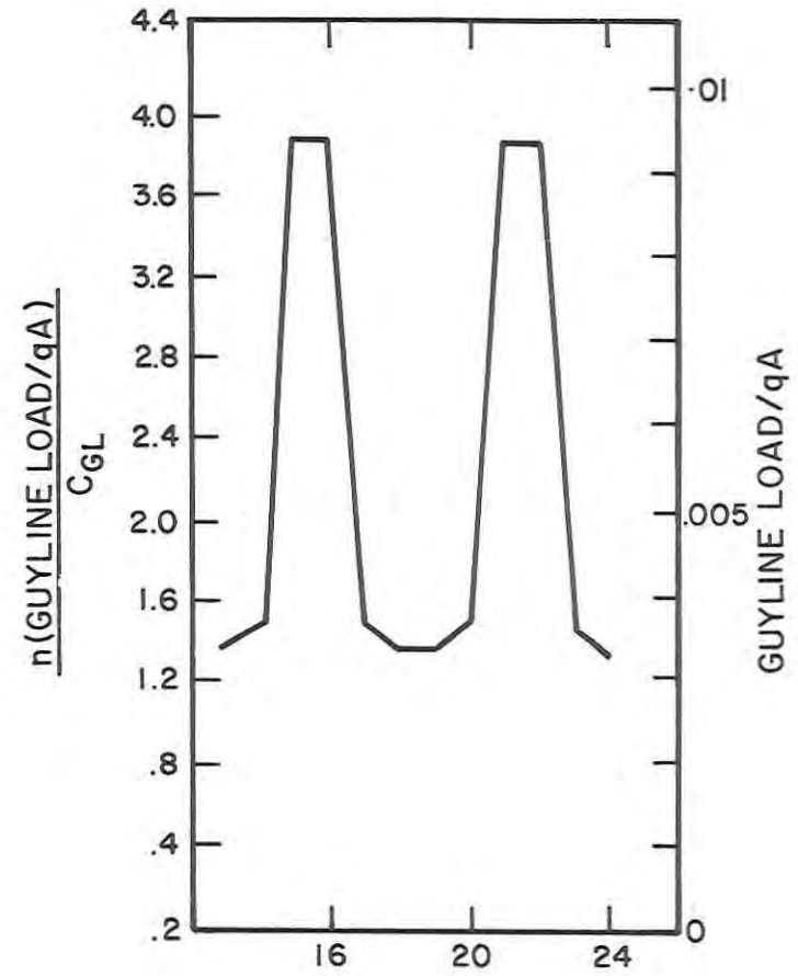
(b) GUYLINE LOAD
