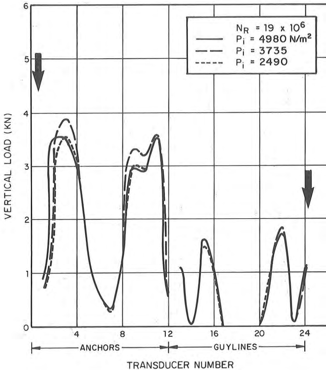
FIG. 14c. DISTRIBUTION OF ANCHOR AND GUYLINE LOAD AT \theta = \pi/2 .
