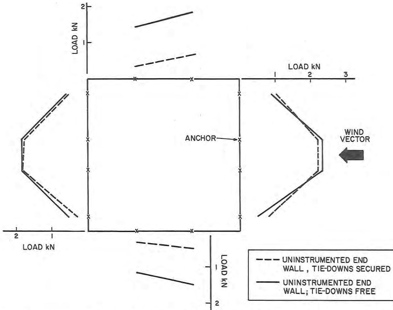
FIG. 11. COMPARISON OF ANCHOR LOADS WITH AND WITHOUT END-WALL GROMMETS ATTACHED TO GROUND PLANE.
