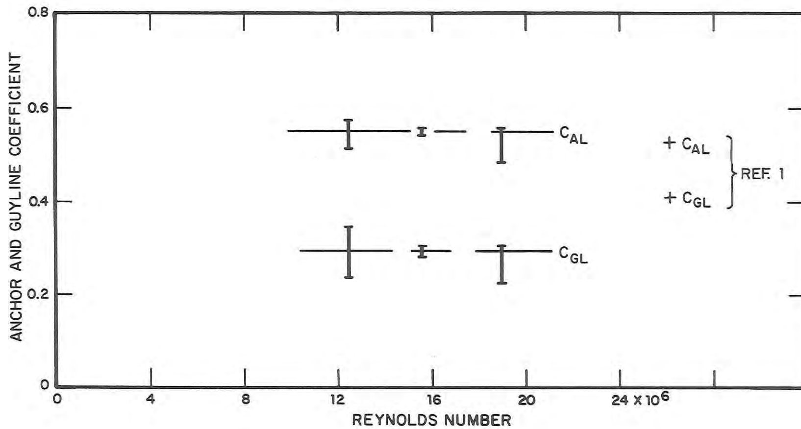
FIG. 13. ANCHOR AND GUYLINE COEFFICIENTS AS A FUNCTION OF REYNOLDS NUMBER.
