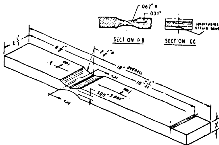
Figure 6 Low-Cycle Fatigue Specimens
