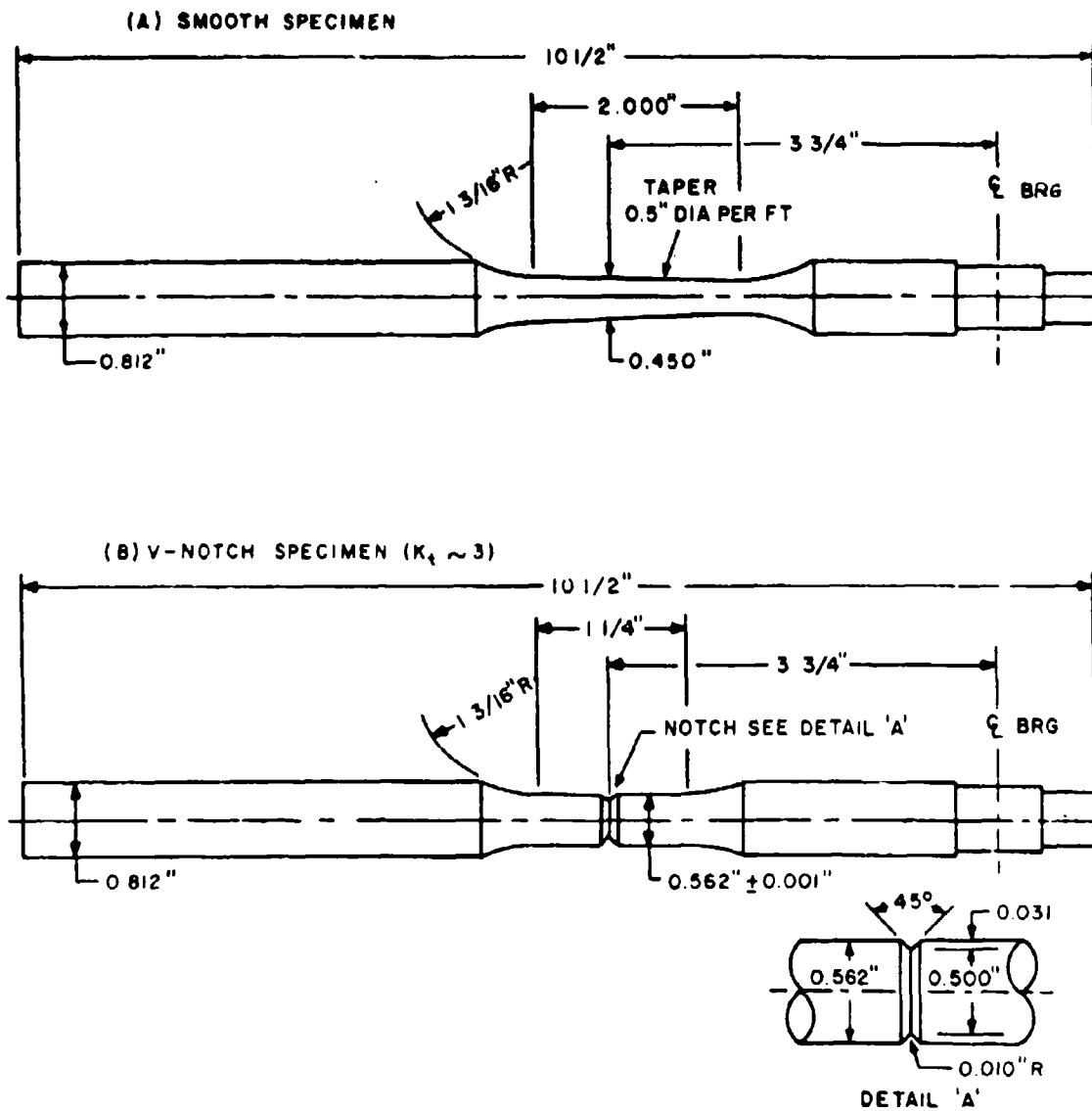
Figure 5 High-Cycle Fatigue Specimens
