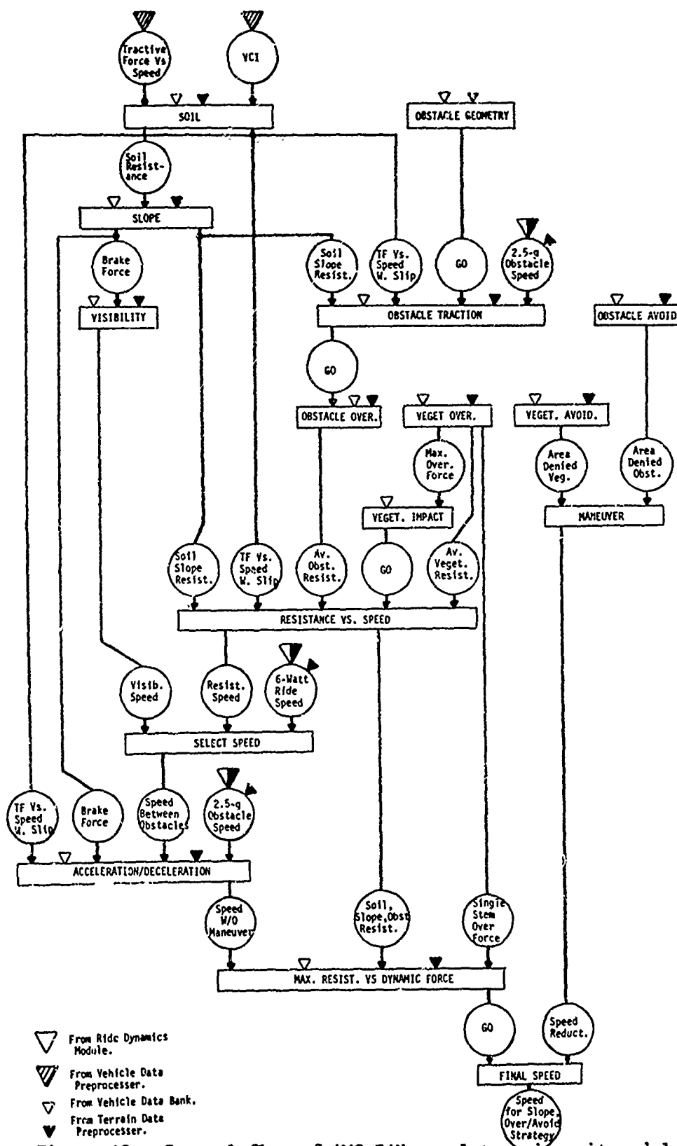
Figure A2. General flow of AMC-74X areal terrain unit module (single loop)
