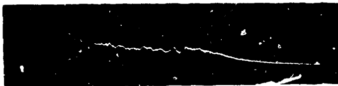
Bird impact; center line pressure transducer filtered output; shot no. 5133; velocity 104 m/s
