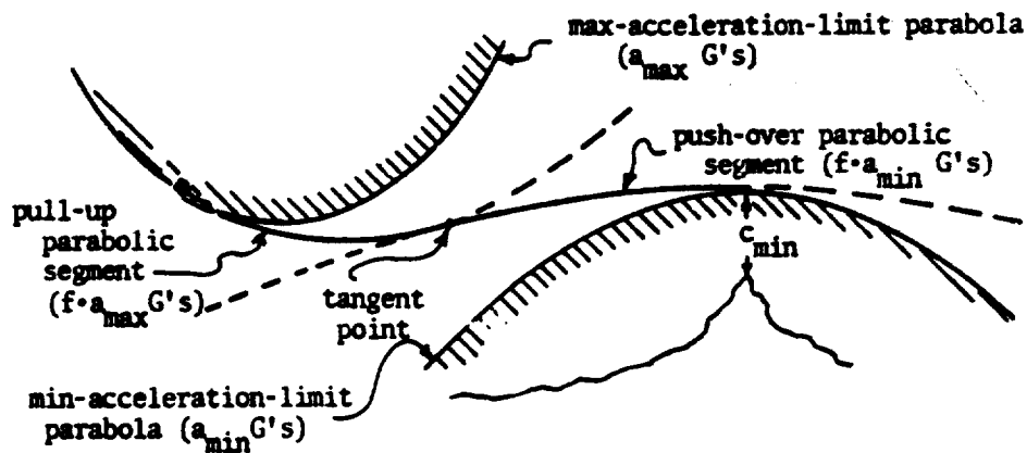
Figure 2-7 ADLAT System Path
