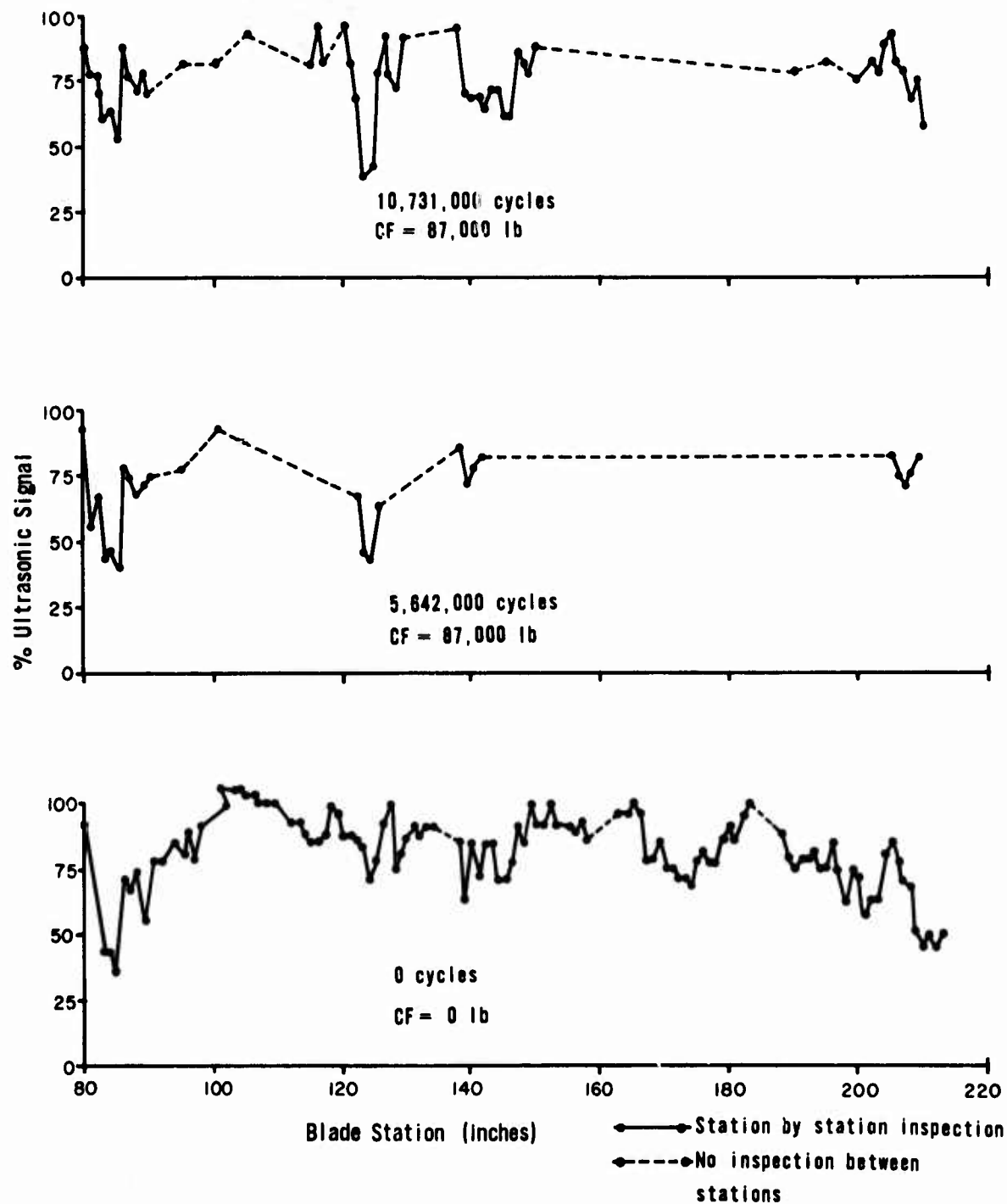
Figure 19. Ultrasonic histogram of test specimen No. 3.
