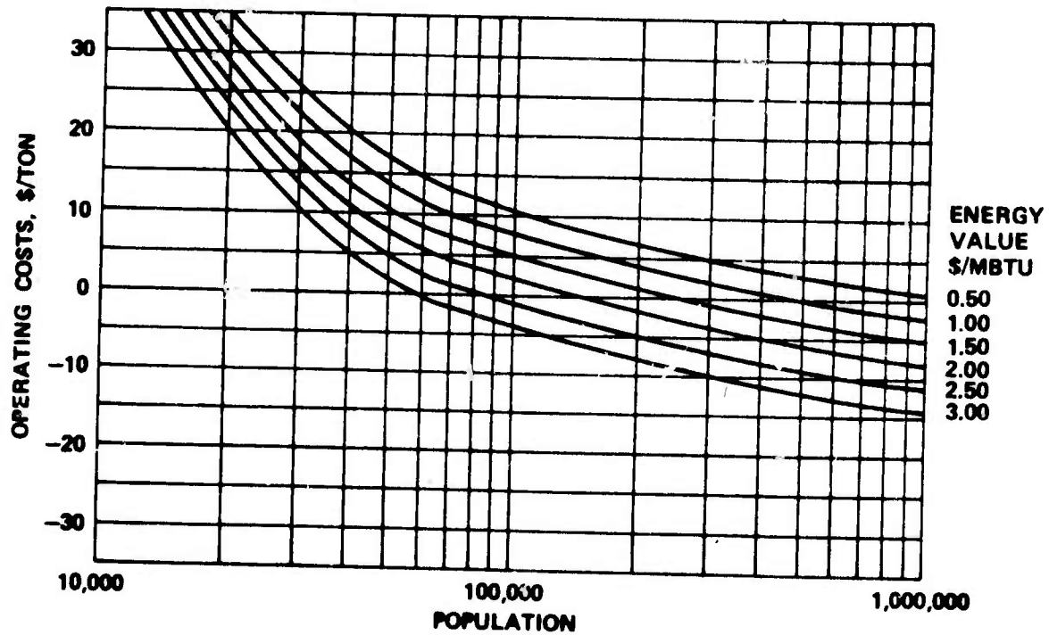
FIGURE 10. Net Operating Costs of Solid Waste Facility with Material Recovery and Conversion of Organic Fraction to Polymer Gasoline.
