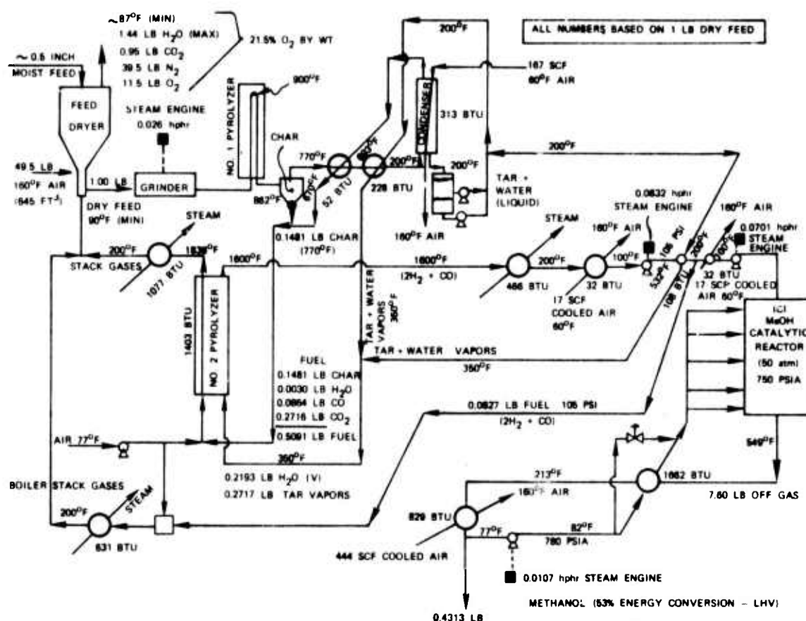
FIGURE 6. Methanol Flow Sheet No. 2.
