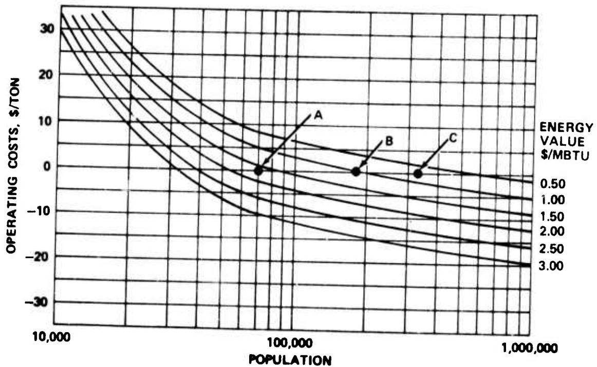
FIGURE 12. Net Operating Costs of Solid Waste Facility with Material Recovery and Conversion of Organic Fraction to Oil or Gas.
