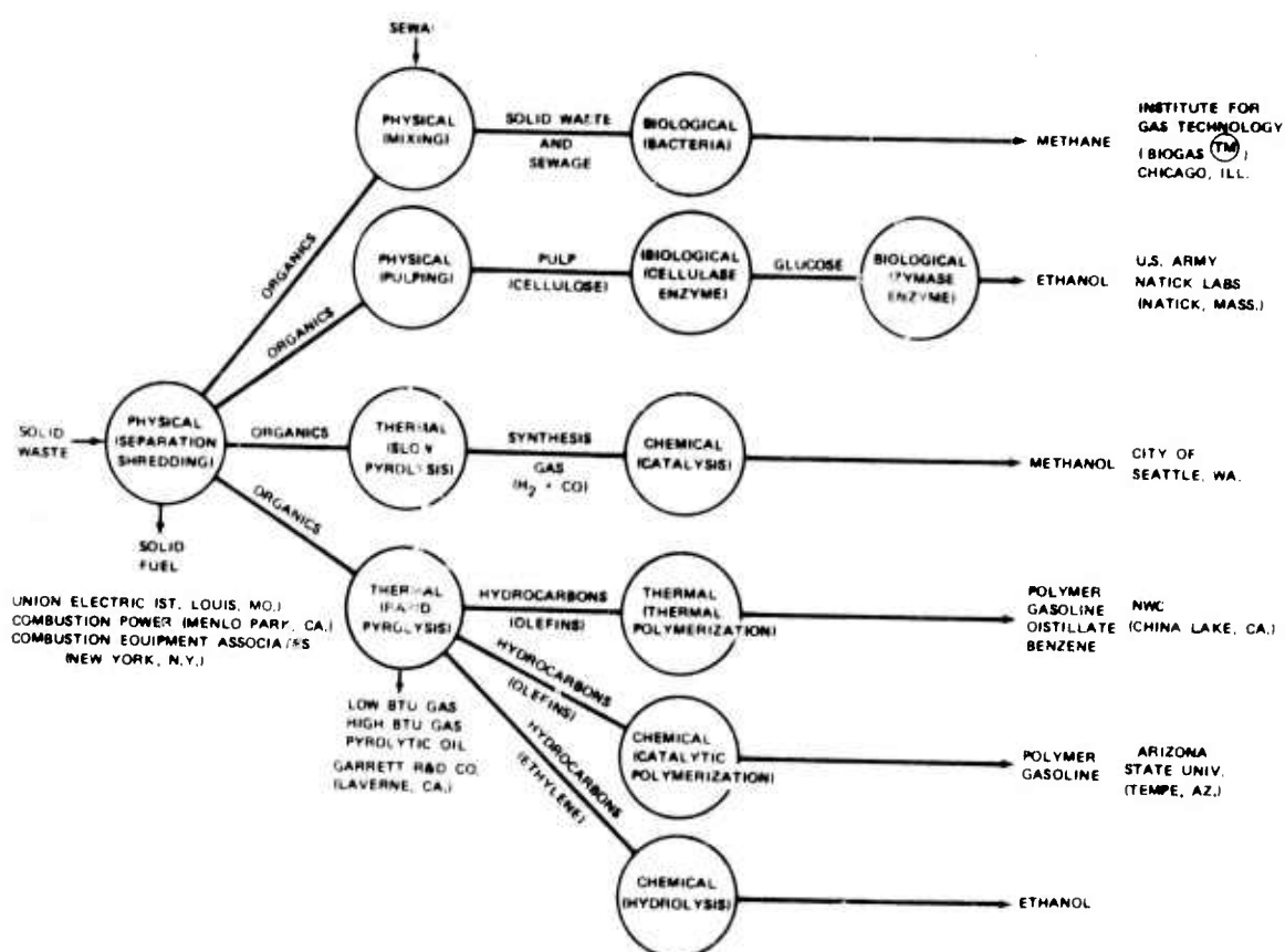
FIGURE 4. Process Routes to Alternate Fuels from Solid Waste.
