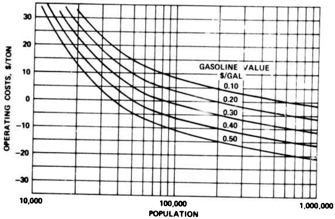
FIGURE 9. Net Operating Costs of Solid Waste Facility with Material Recovery and Conversion of Organic Fraction to Polymer Gasoline.
