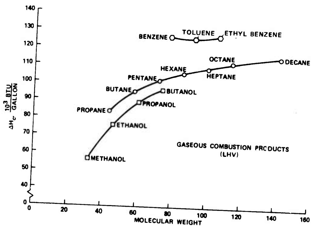
FIGURE 1. Volumetric Heat of Combustion Versus Molecular Weight.
