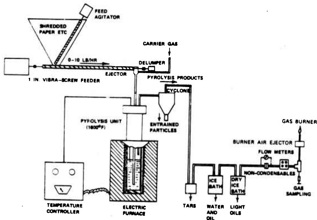
FIGURE 14. Pyrolysis Schematic.
