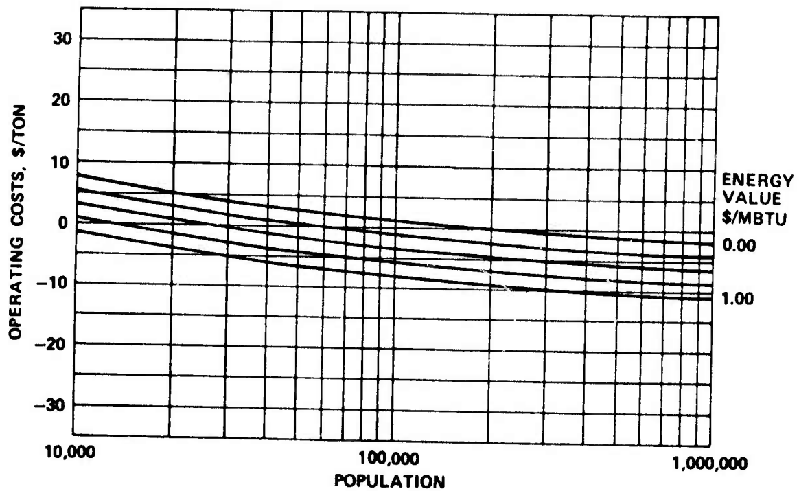
FIGURE 11. Net Operating Costs of Solid Waste Facility with Material Recovery and Use of Organic Fraction as Substitute Coal.
