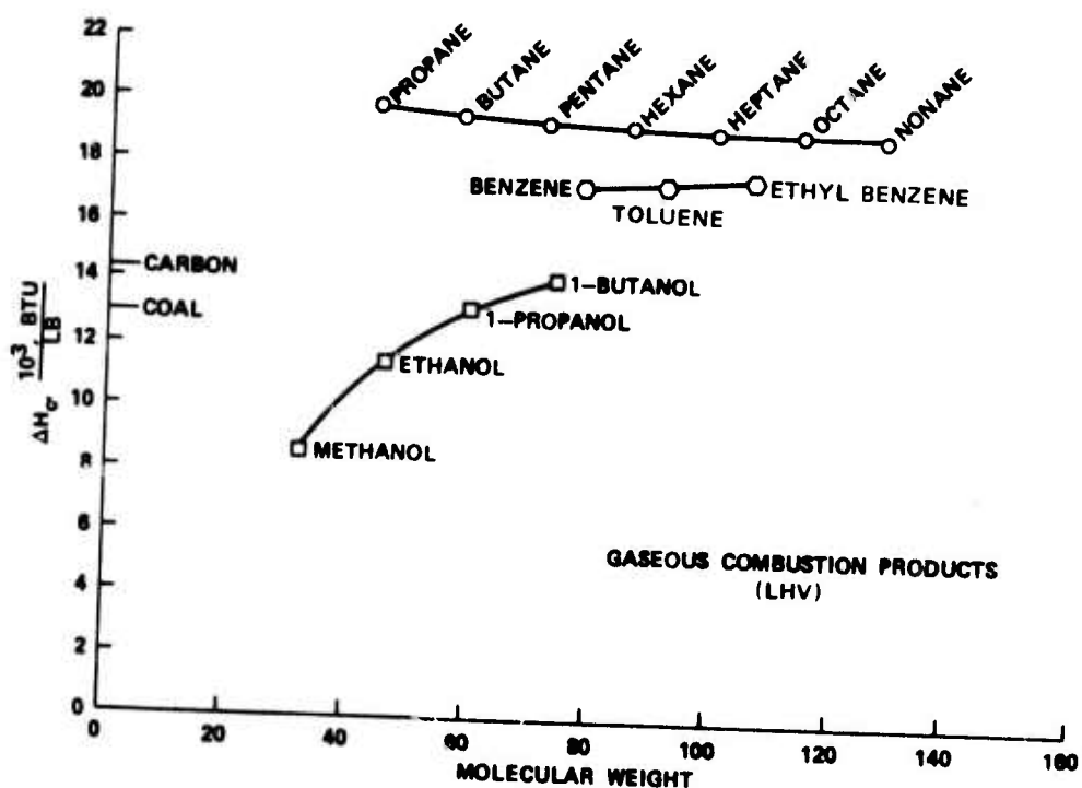
FIGURE 2. Gravimetric Heat of Combustion Versus Molecular Weight.
