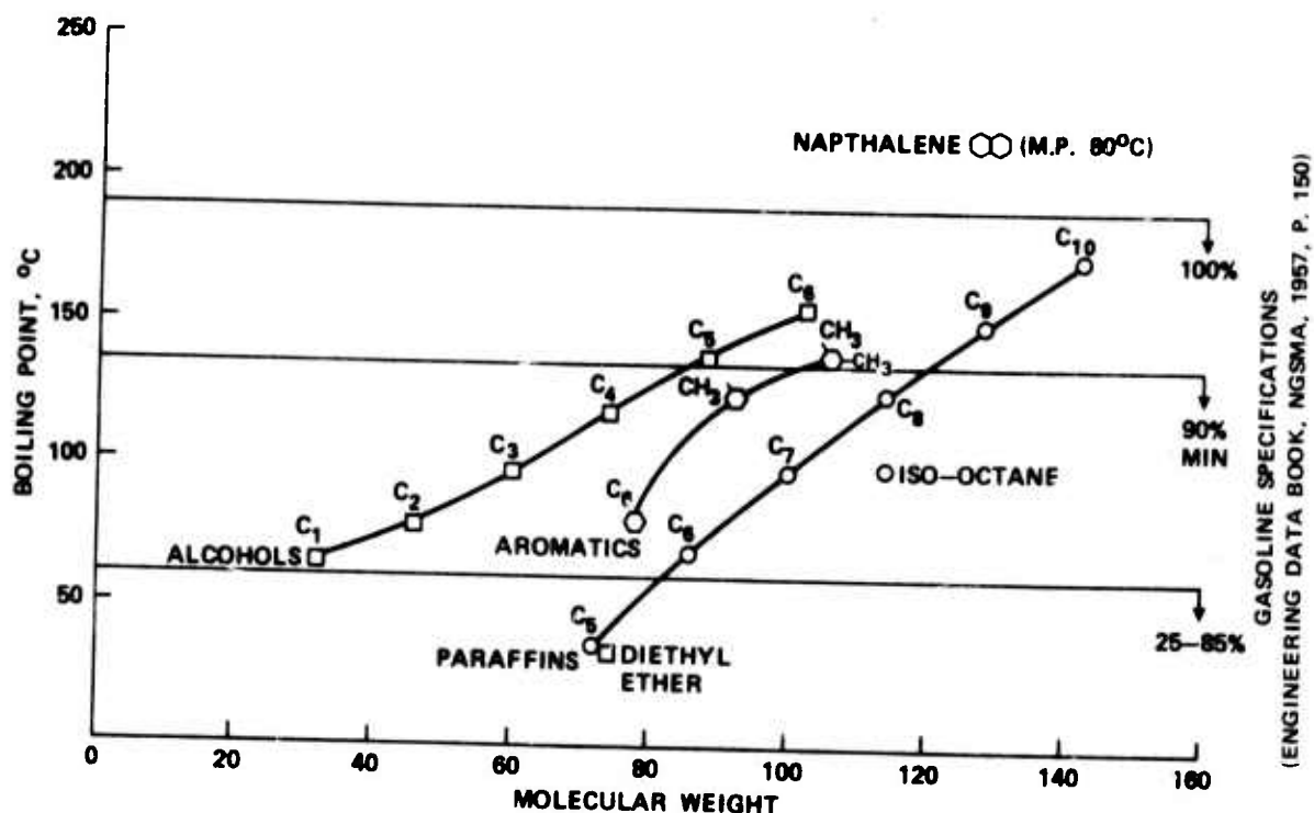
FIGURE 3. Boiling Point Versus Molecular Weight (Ref.: Lange's).
