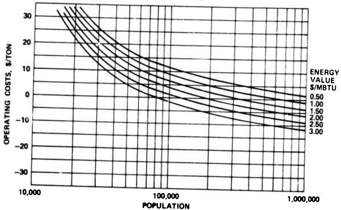
FIGURE 8. Net Operating Costs of Solid Waste Facility with Material Recovery and Conversion of Organic Fraction to Methanol.
