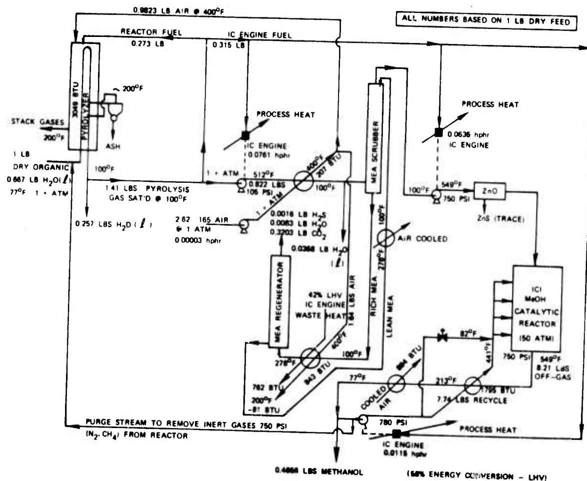
FIGURE 5. Methanol Flow Sheet No. 1.
