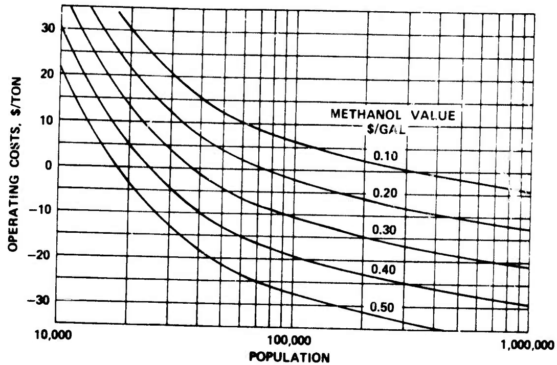
FIGURE 7. Net Operating Costs of Solid Waste Facility with Material Recovery and Conversion of Organic Fraction to Methanol.
