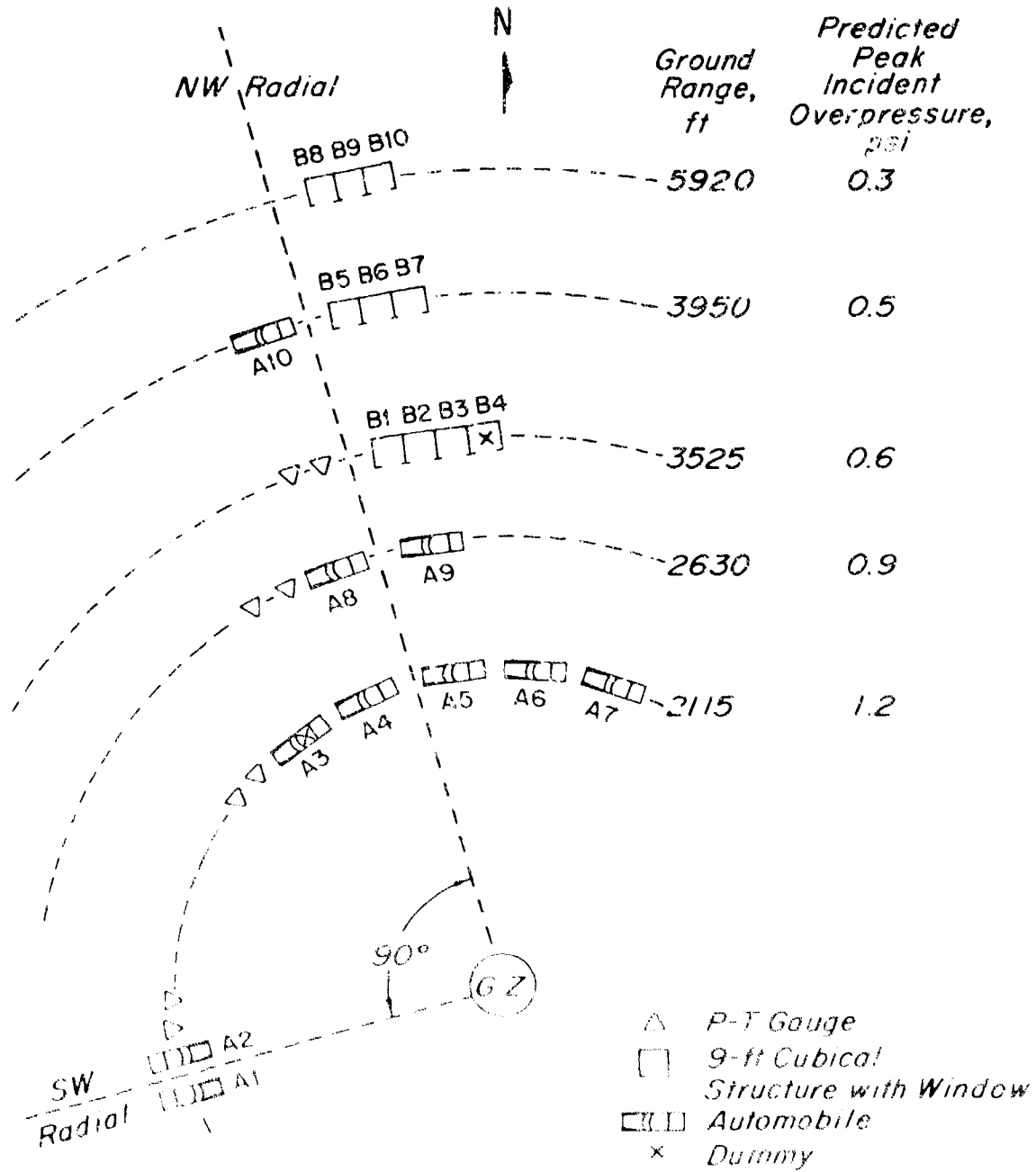
FIGURE 1. Car Field Layout for the Eskimo III Test
