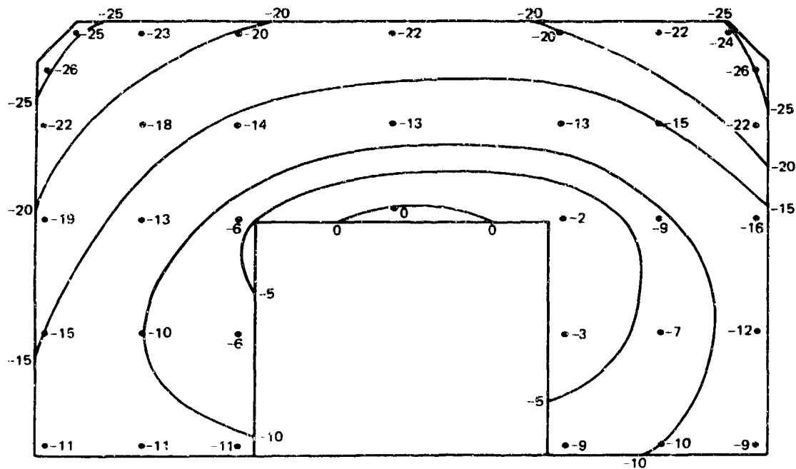
FIGURE 45. Headwall Movement, Igloo D. Minus values indicate movement outward, toward the donor; one point (above door) showed no movement. Units shown are hundredths of feet.
