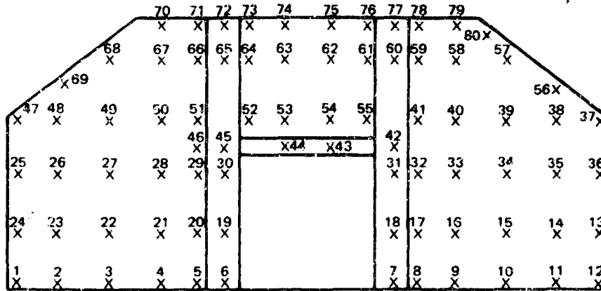
FIGURE 41. Position Key for Headwall Deformation Measurements, Igloo B.
