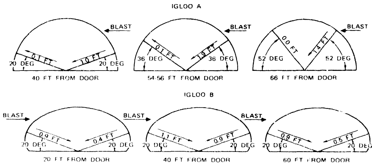
FIGURE 48. Maximum Static Arch Movements at Blast Side of Arch. Movements at corresponding positions on leeward side are also shown.
