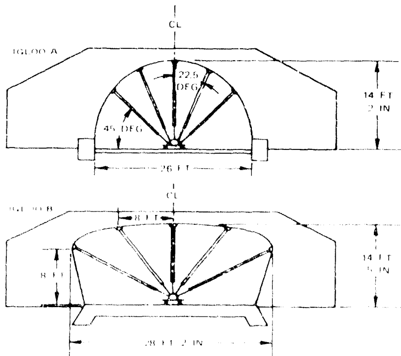
FIGURE 4. Igloos A and B. Dots - Relative Slopes and Locations of Displacement Measuring Apparatus on Each
