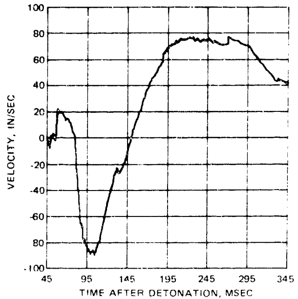
(b) Velocities derived from accelerometer record.
