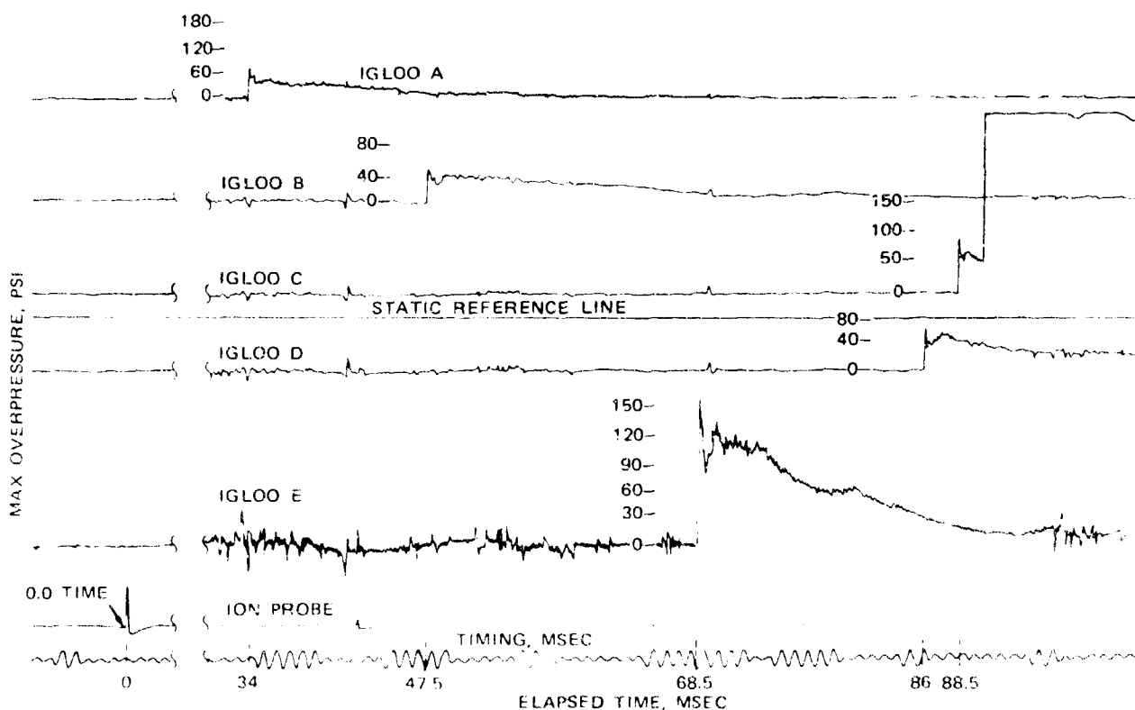
FIGURE 32. Kistler Piezoelectric Blast Gauge Data. Time of blast arrival versus peak overpressure. Gauges located in the right headwall of each igloo.
