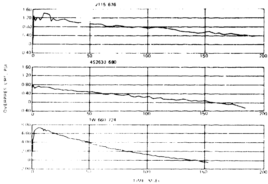
FIGURE 35. Data Plots for BRI Gauges on the Southwest Leg at 2,115 and 2,630 Feet, and the Northwest Leg at 660 Feet.
