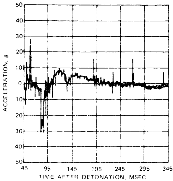
(a) Accelerometer record.
