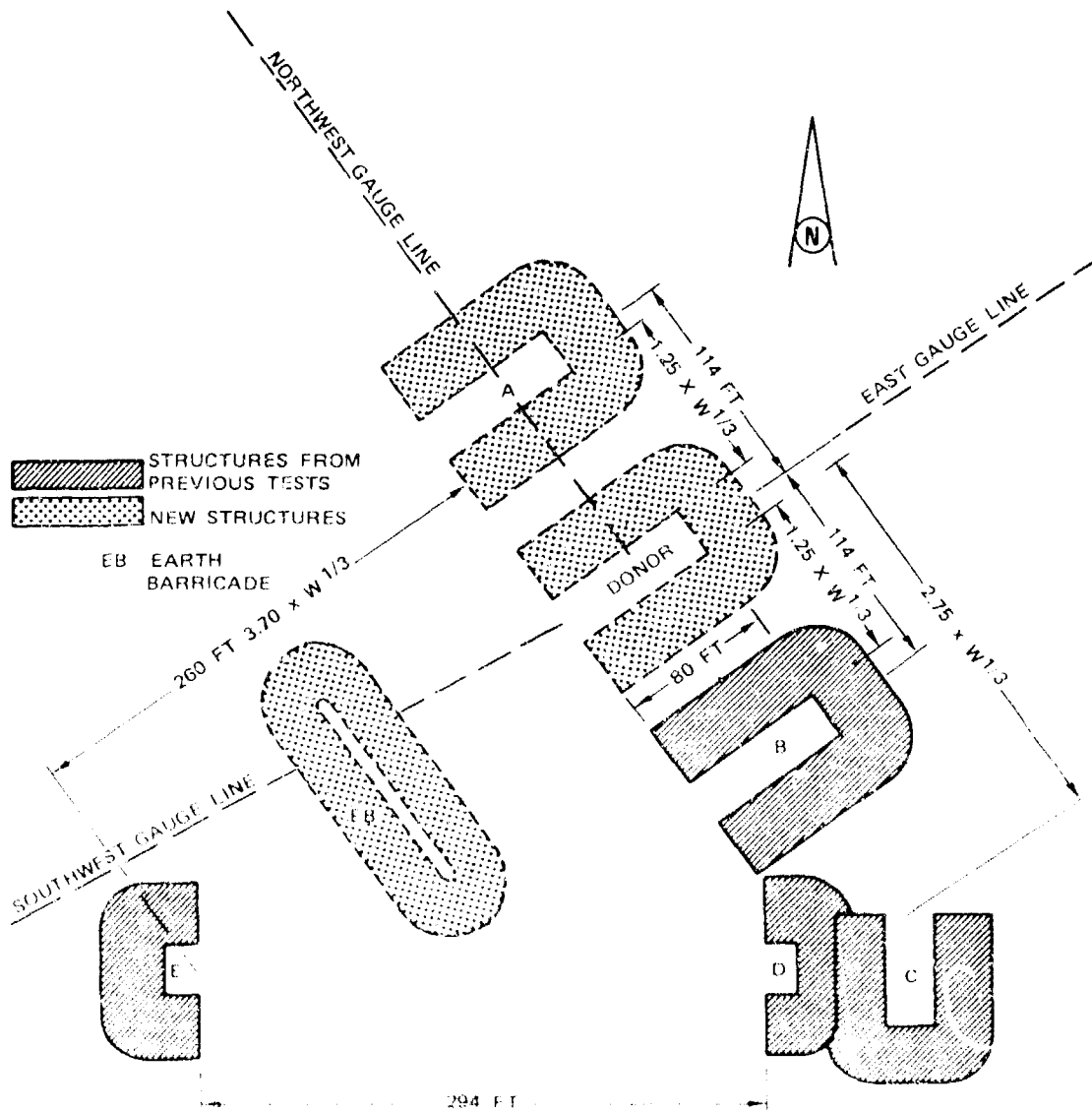
FIGURE 2. Layout of Test Structures for ESKIMO III Magazine Separation Test. A, B, C, D, and E indicate acceptor igloo destinations.
