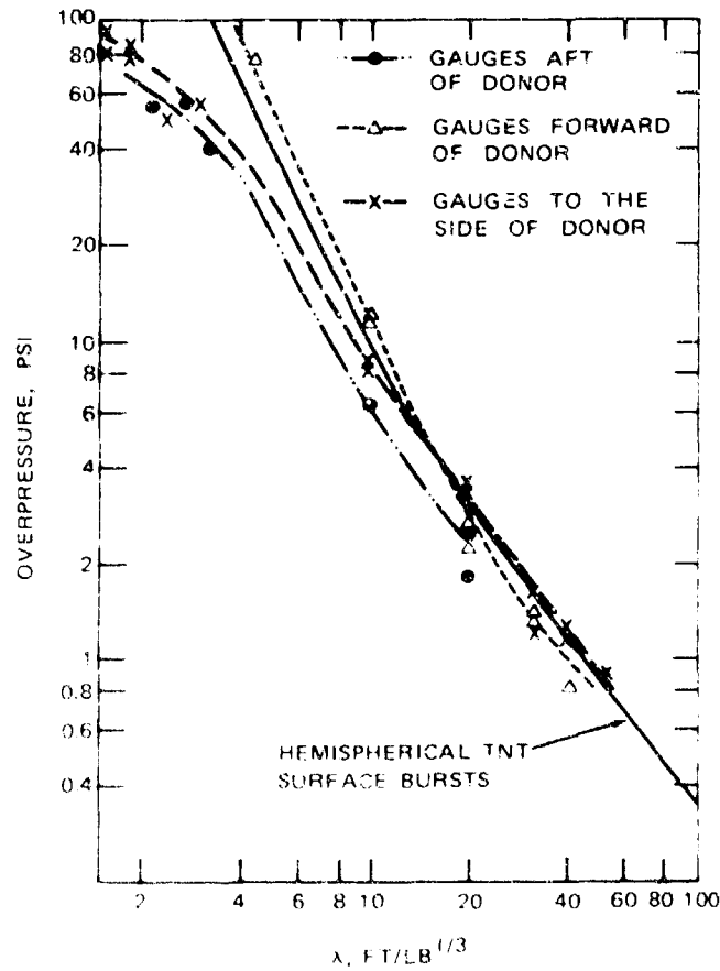
FIGURE 27. Plot of Overpressure Versus Scaled Distance (a) Compare ENKIMO III Blast Data With Standard TNT Blast Data. Assumed effective explosive weight, W = 295,000 pounds.
