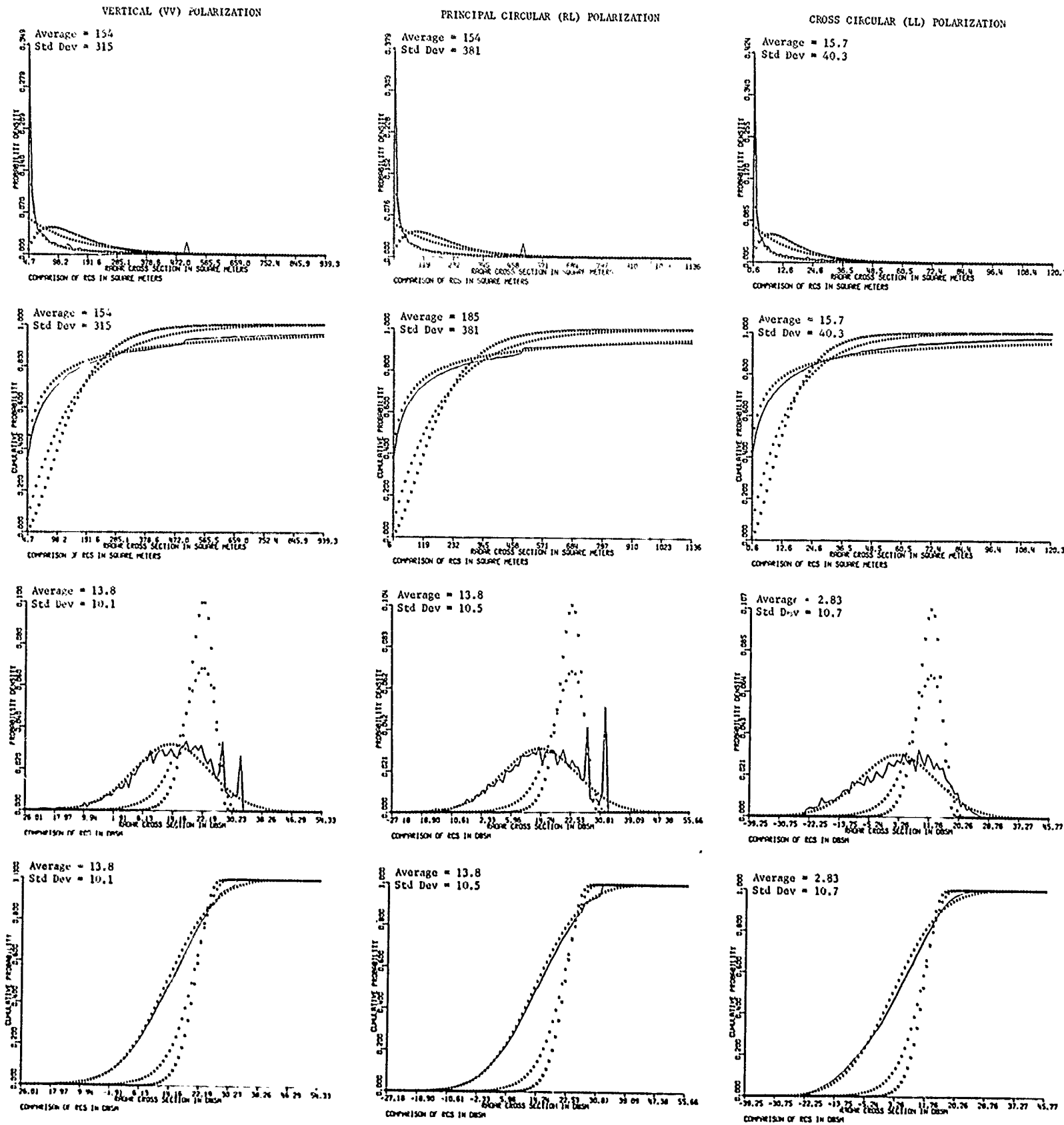
Figure 23. Comparison of measured data and theoretical models for aspect angles within 15° of normal to the roll axis.
