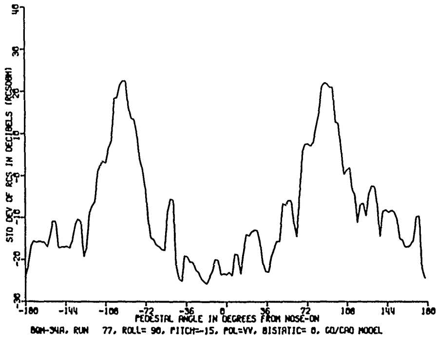
Figure 16. Average and standard deviation of measured RCS, -15^\circ pitch, 90^\circ roll.
