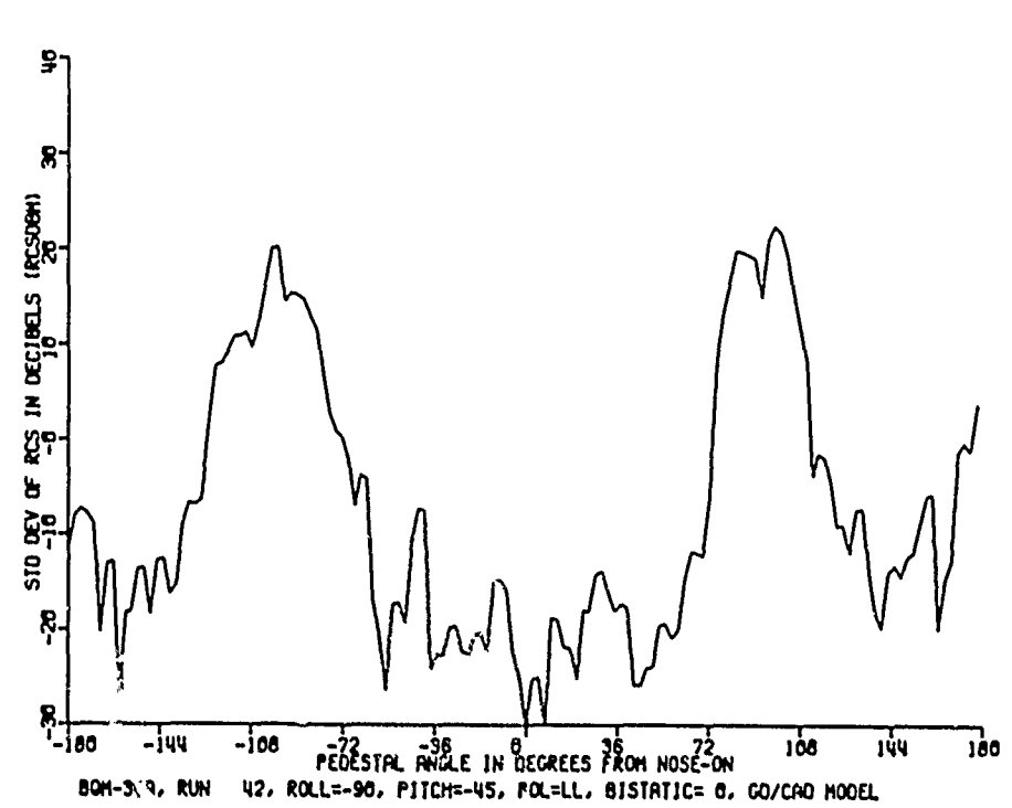
PEDESTAL ANGLE IN DEGREES FROM NOSE-ON BQM-34A, RUN 42, ROLL=-90, PITCH=-45, POL=LL, BISTATIC= 0, GO/CAO MODEL
