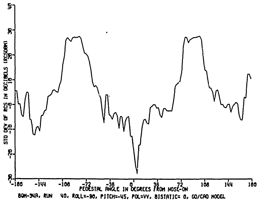
Figure 10. Average and standard deviation of measured RCS, -45^\circ pitch, -90^\circ roll.
