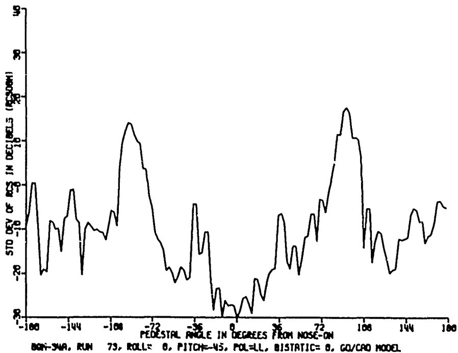
Figure 15. Average and standard deviation of measured RCS, -45° pitch, 0° roll.
