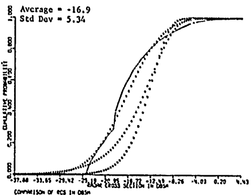
Figure 21. Comparison of measured data and theoretical models for aspect angles greater than 30° and less than 60° from nose-on.
