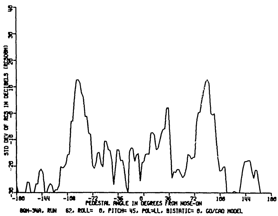
Figure 13. Average and standard deviation of measured RCS, 45° pitch, 0° roll.
