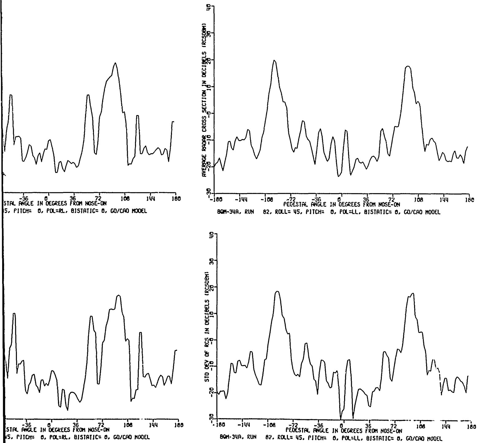
Figure 17. Average and standard deviation of measured RCS, 0° pitch, 45° roll.
