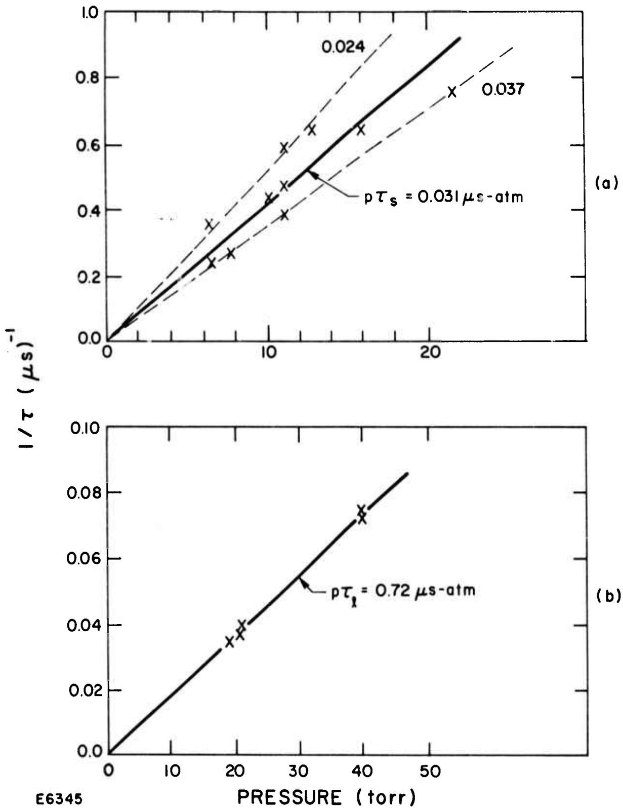
Fig. 12 1/\tau vs Pressure Plot for the (a) Short and (b) Long Time Constants at 7.8 \mu\text{m}
