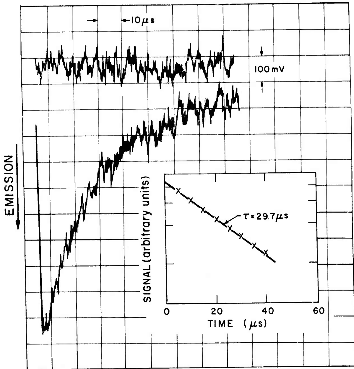
Fig. 14 Fluorescence Scan at 4.5 μm
