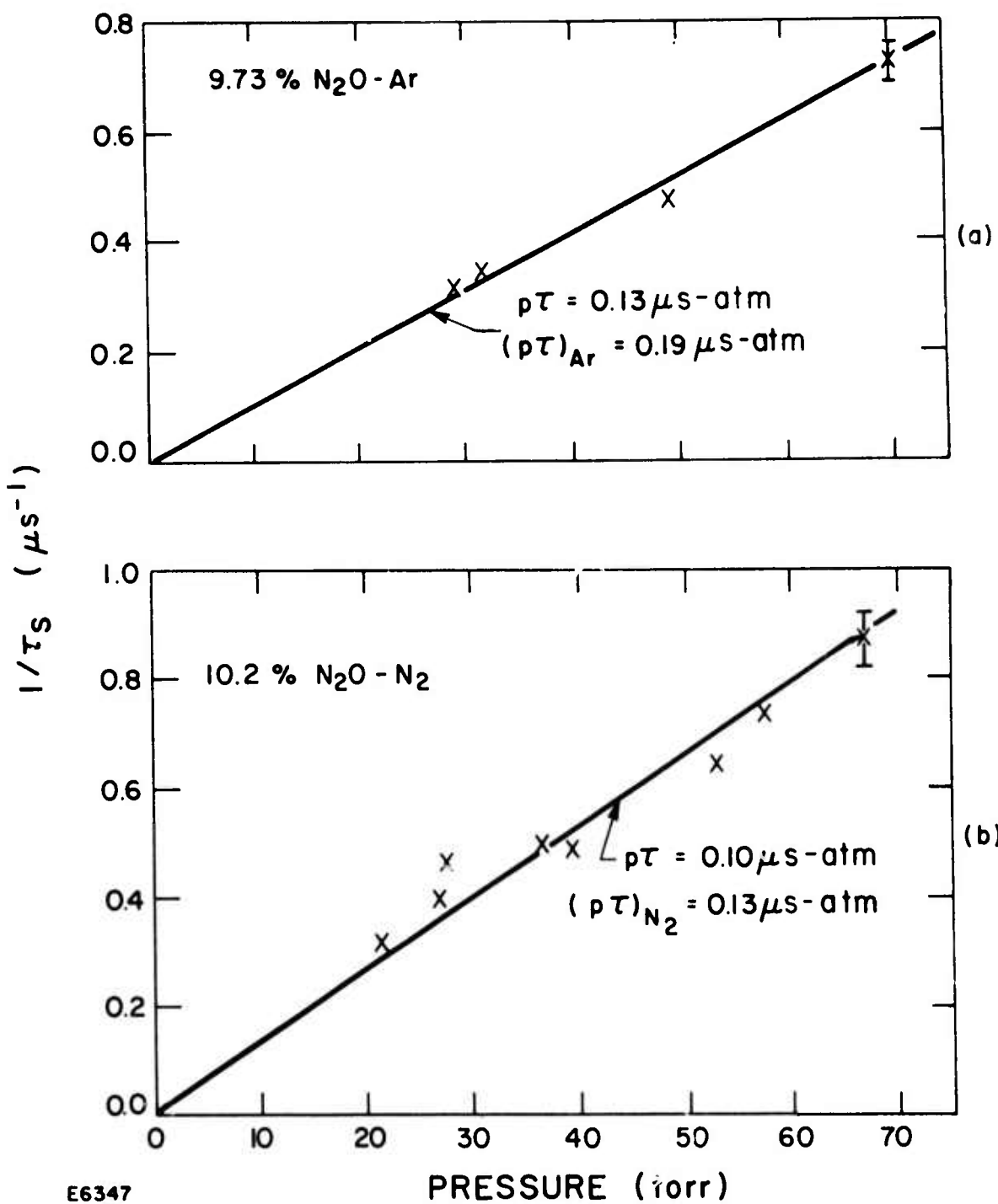
E6347 Fig. 17 (a) Short Time Constant (V-V) Measurements of 9.73 Percent N_2O in Ar Mixture. Plot of 1/\tau_s vs Pressure (b) Short Time Constant (V-V) Measurements of 10.2 Percent N_2O in N_2 Mixture. Plot of 1/\tau_s vs Pressure
