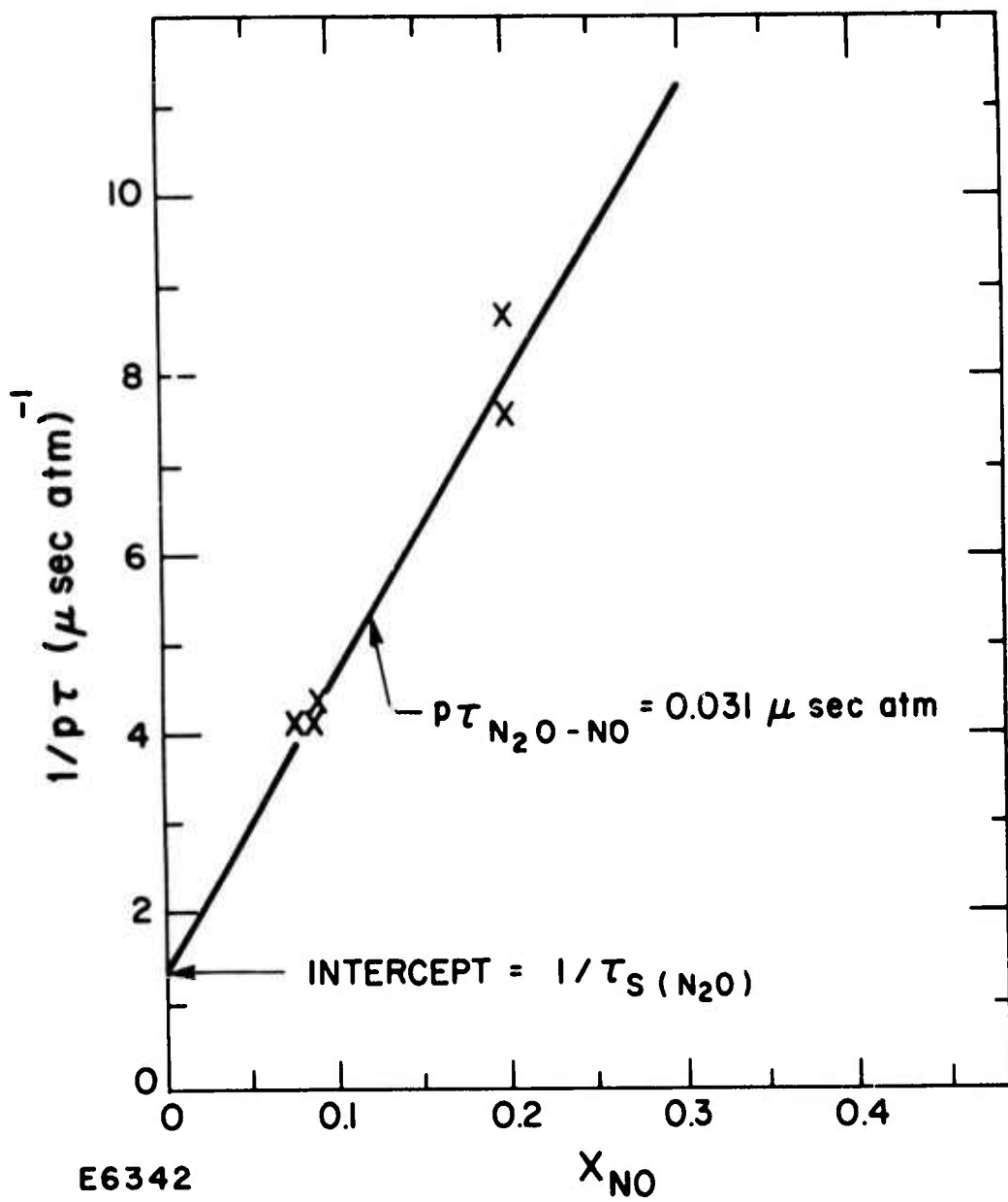
Fig. 20 Plot of 1/p\tau vs Mole Fraction of No in Mixtures of \text{N}_2\text{O} -NO
