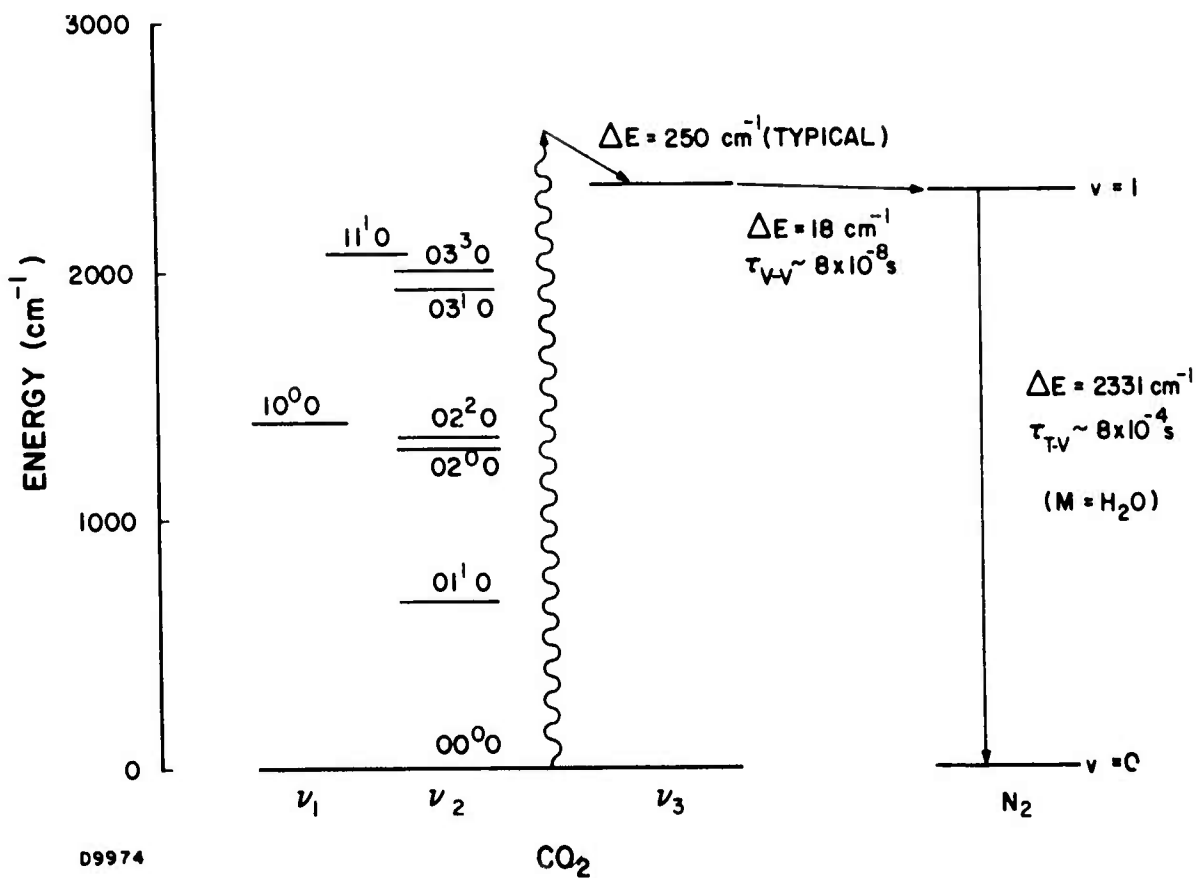
Fig. 3 Kinetics of Absorption of DF Laser Radiation by CO 2
