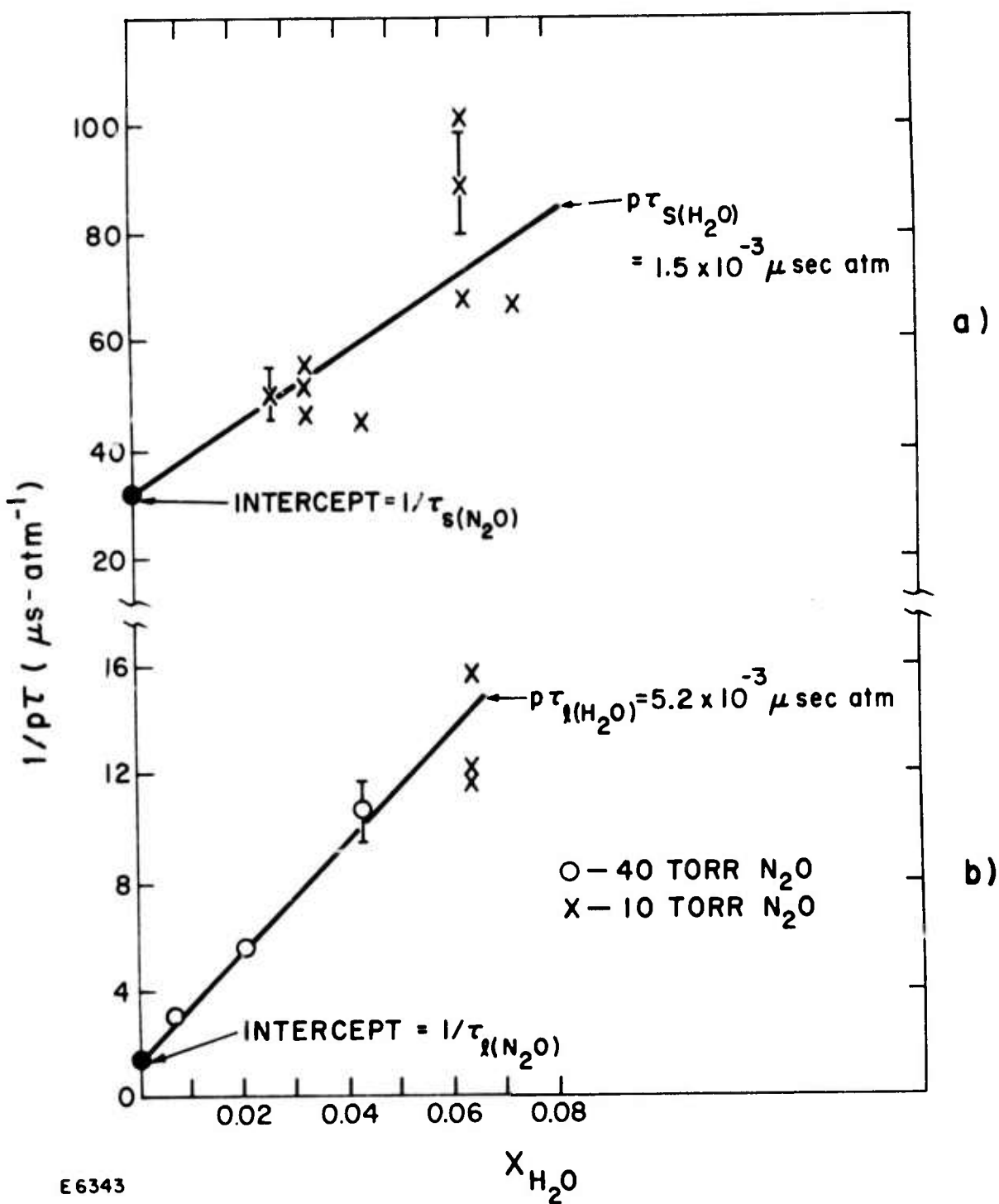
Fig. 18 (a) Short Time Constant (V-V) Measurements of N_2O - H_2O Mixtures. Plot of 1/p\tau_s vs Mole Fractions of H_2O ( X_{H_2O} ) (b) Long Time Constant (V-T) Measurements of N_2O - H_2O Mixtures. Plot of 1/p\tau_l vs ( X_{H_2O} )
