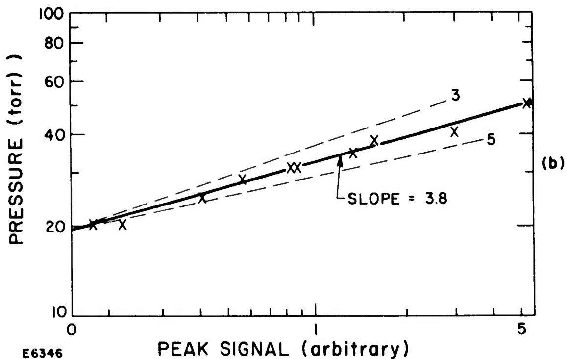
Fig. 15 (a) Observed Peak 4.5 \mu\text{m} Fluorescence Signal (Arbitrary Units) vs \text{N}_2\text{O} Pressure
