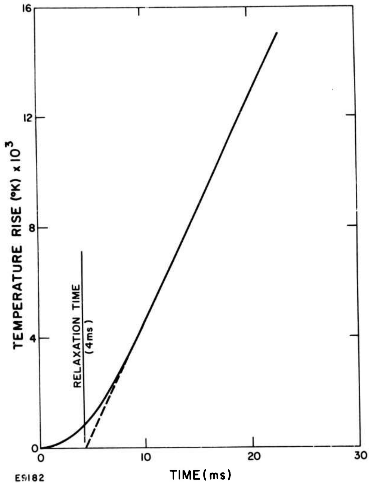
Fig. 21 Thermal Response of the Atmosphere to DF Laser Radiation ( 10^5 \text{W/cm}^2 on the 3 P(9) Transition) under Sea Level, Low Humidity Conditions
