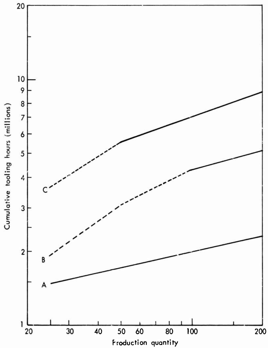
Fig. C-3 — Cumulative tooling hours for three airframe programs
