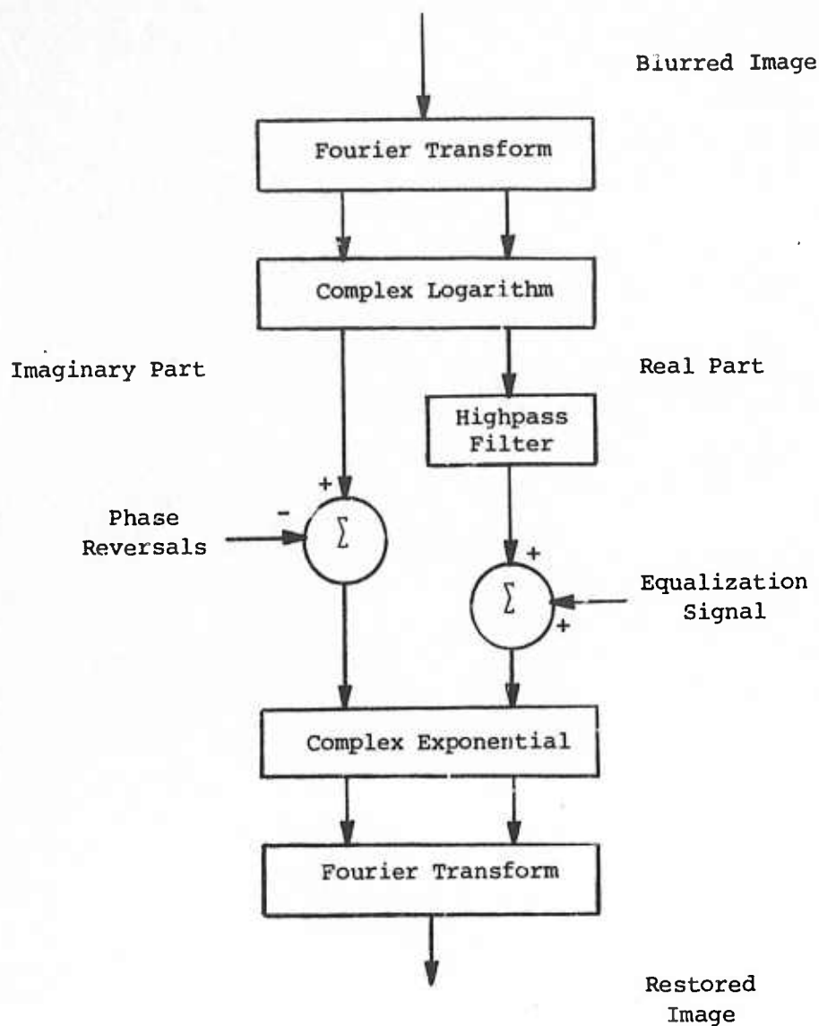
Figure 1.1 -- A deblurring mechanism suggested by the texture equalization property.
