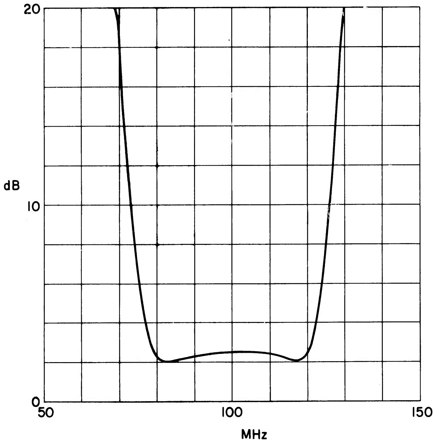
FIG. 8--Transducer response.
