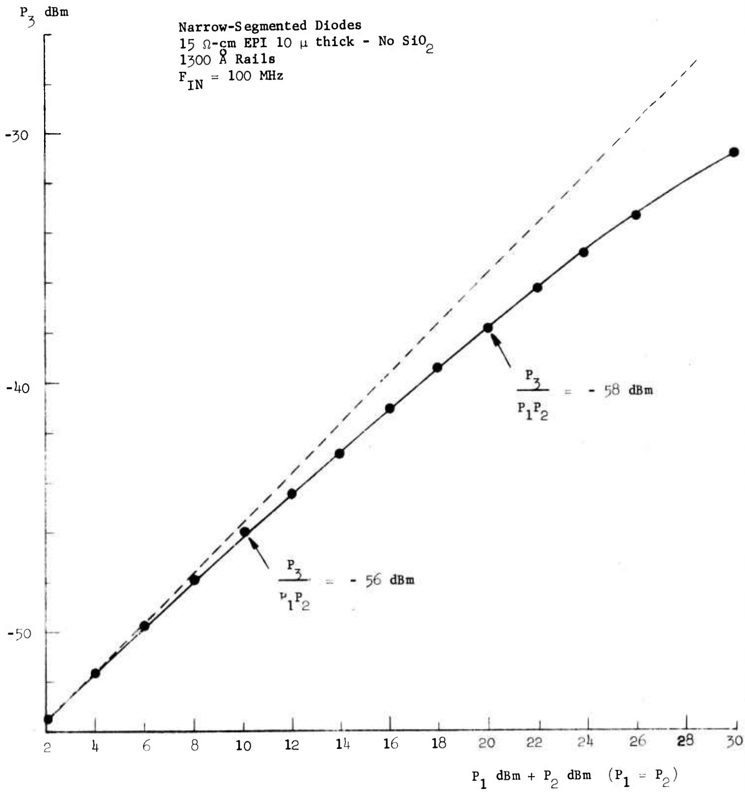
FIG. 16--Output power versus input power.
