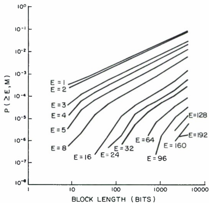
Figure 6. Probability of at Least E Errors in an M Bit Block — 9600 b/s Data
